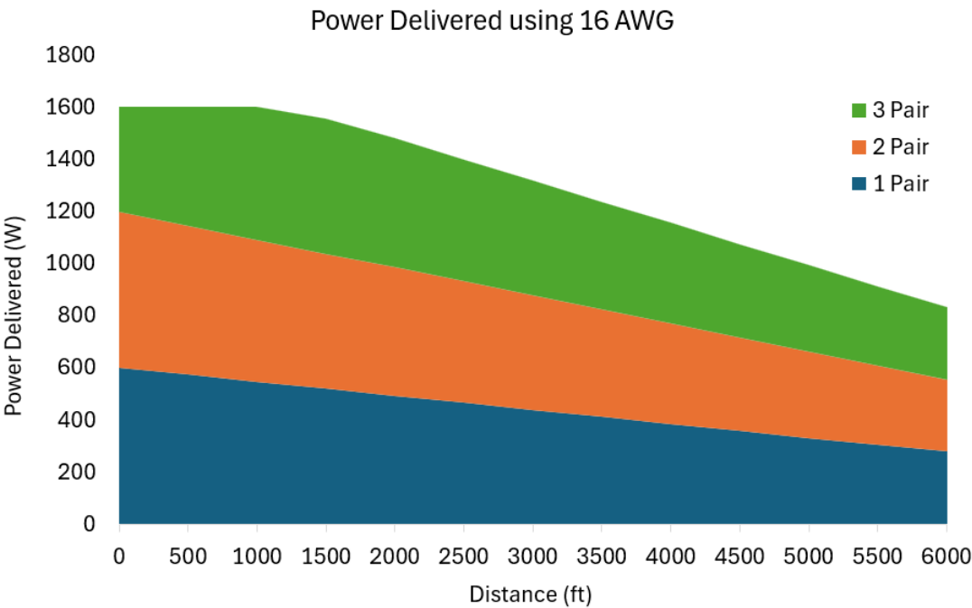
Wattage Delivered Relative to Distance Using 16 AWG Multiconductor Cable and Pair Count
