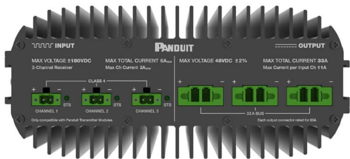
Input/Output Face of Receiver
