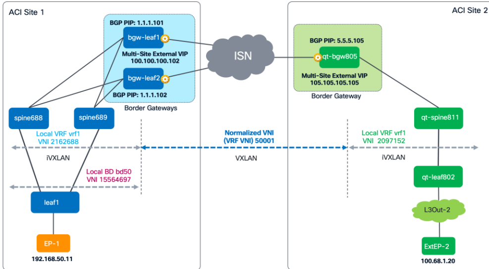
Figure 262. Data plane North-South Communication Across ACI Sites with Non-stretched BD
