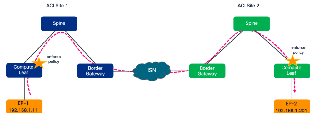
Figure 112. Intra-Subnet communication policy enforcement
