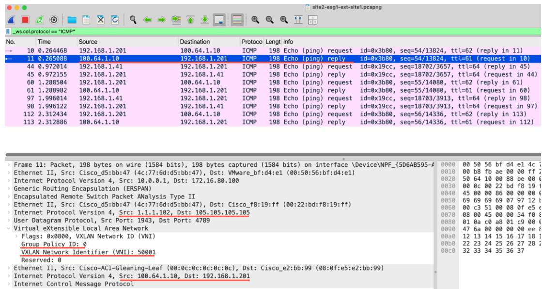
Figure 236. ICMP reply from ExtEP-1 (100.64.1.10) to EP-2 (192.168.1.201)
