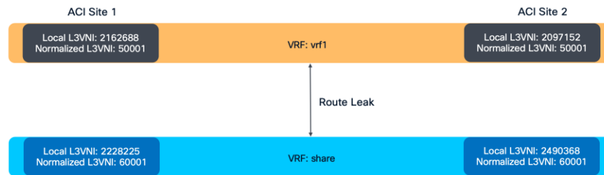
Figure 347. Route Leak diagram
