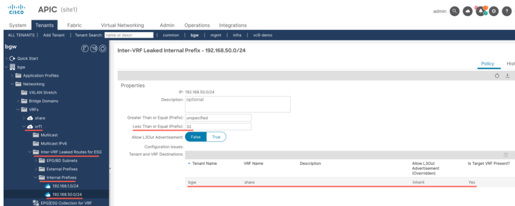
Figure 386. ACI Site 1 leak prefix 192.168.50.0/24 from VRF vrf1 to VRF share
