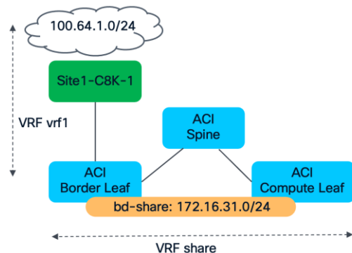
Figure 419. Advertise 172.16.31.0/24 to ACI Site 1 L3Out in VRF vrf1
