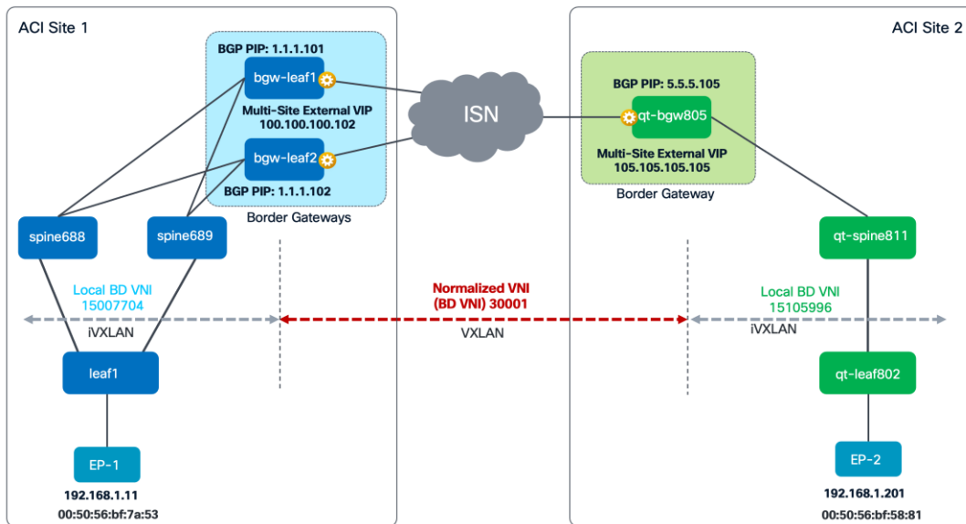
Figure 107. Data plane Bridged Communication across sites
