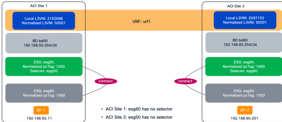
Figure 165. Inter-Subnet Communication Non-stretched BD Multiple ESGs
