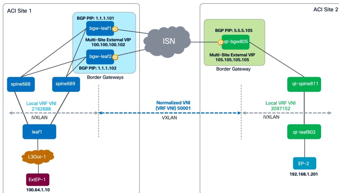
Figure 234. Data plane North-South Communication Across ACI Sites with Stretched BD
