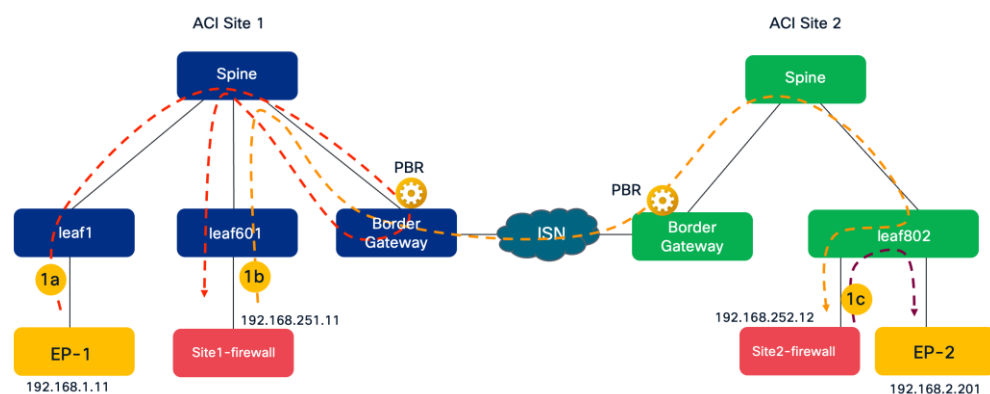
Figure 444. Flow from ACI Site 1 esg1 endpoint to ACI Site 2 esg2 endpoint
