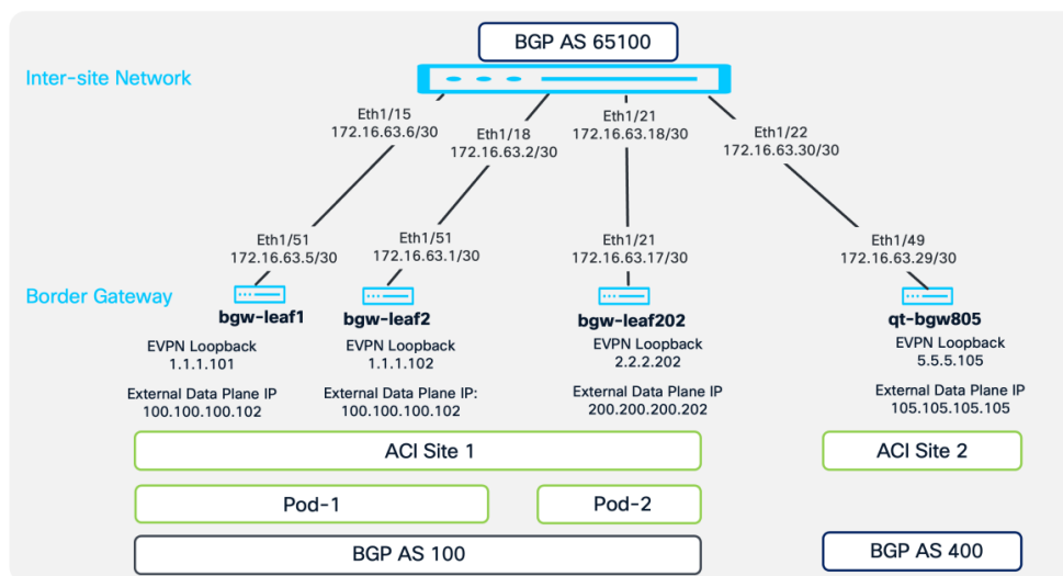
Figure 38. Topology with IP addressing
