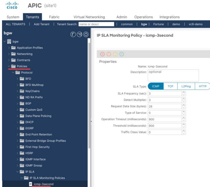
Figure 449. ACI Site 1 IP SLA Monitoring Policy
