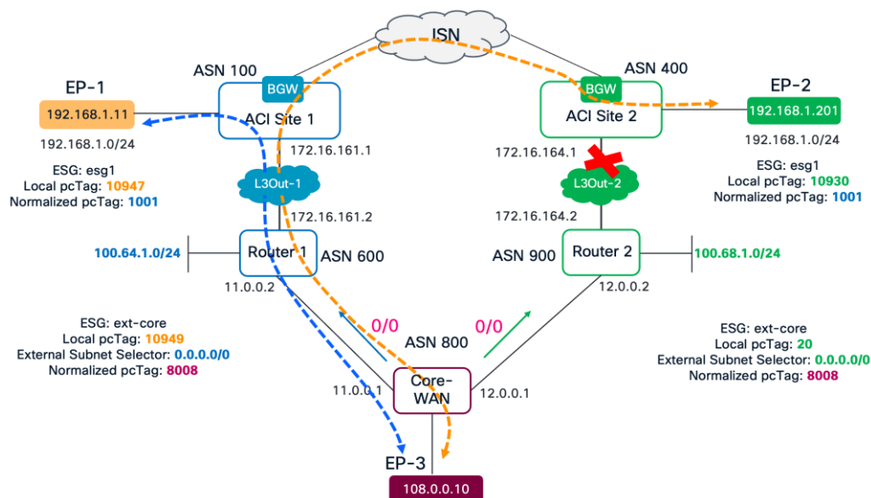
Figure 316. ACI Site 2 traffic failover when L3Out-2 down
