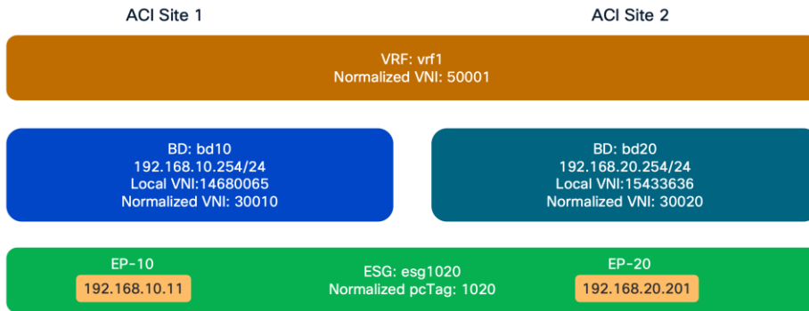
Figure 144. ESG esg1020
