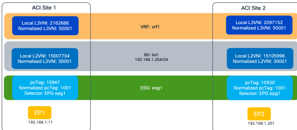
Figure 81. Intra-Subnet Communication
