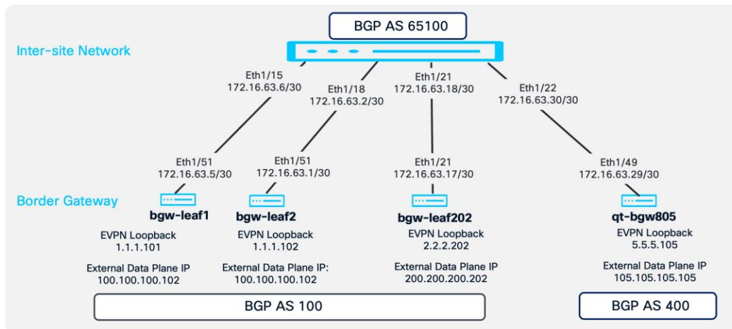
Figure 7. ISN Underlay IP addressing
