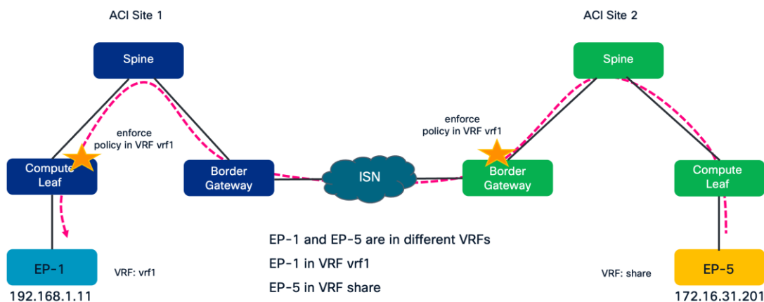
Figure 367. Policy enforcement VRF share to VRF vrf1, from ACI Site 2 to ACI Site 1
