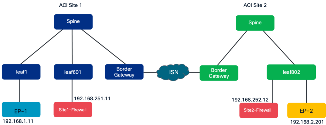
Figure 468. Firewall insertion topology example
