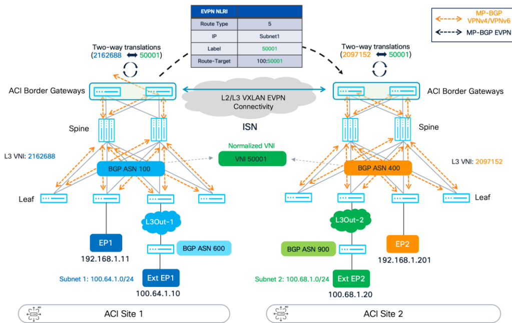
Figure 219. EVPN Type 5 Route exchange across ACI Sites
