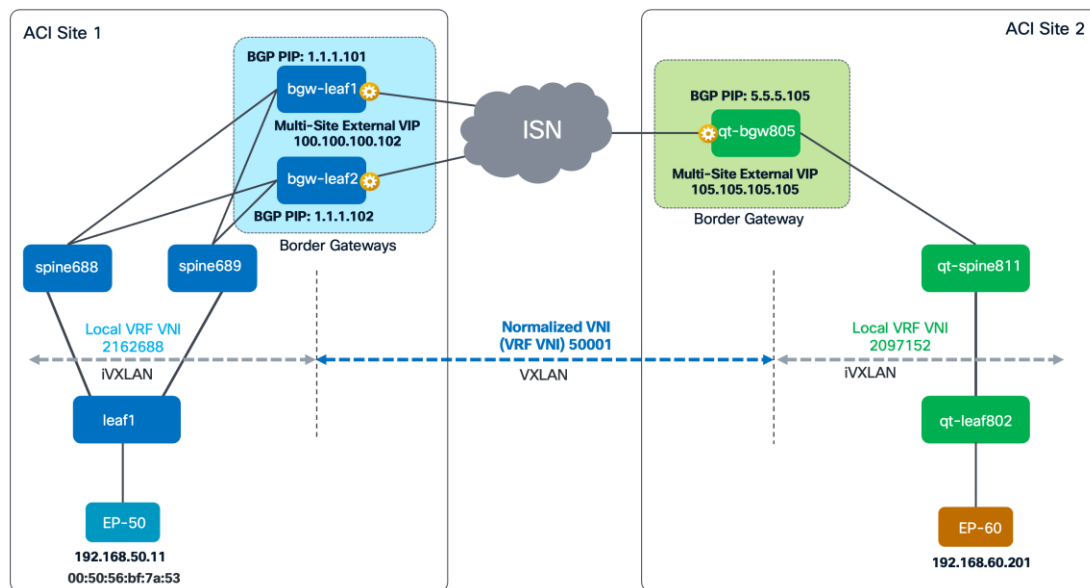
Figure 201. Data plane Inter-Subnet Communication with Non-stretched BDs and Multiple ESGs
