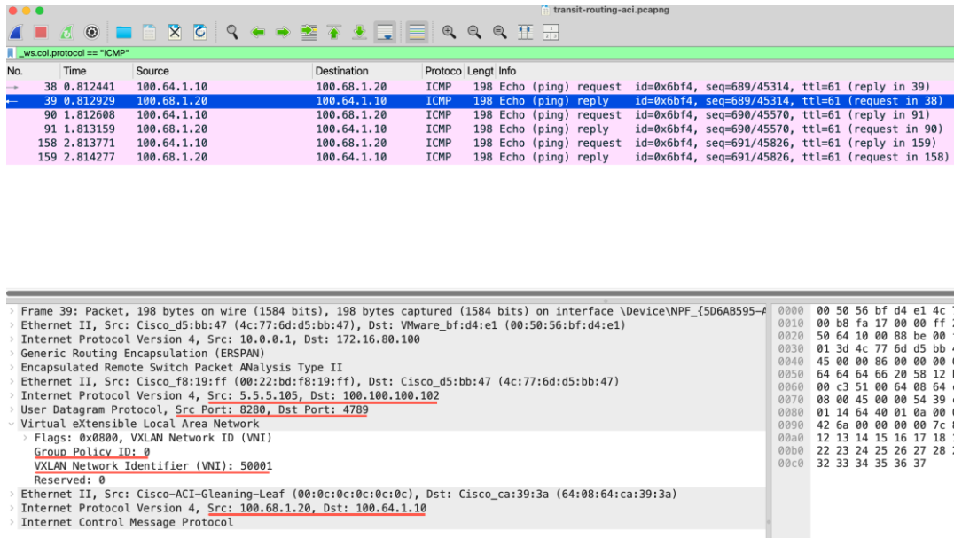
Figure 294. ICMP reply from ExtEP-2 (100.68.1.20) to ExtEP-1 (100.64.1.10)
