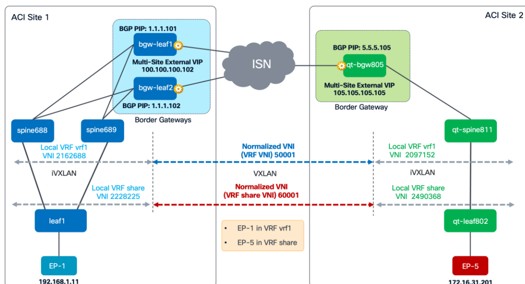
Figure 363. Data plane Shared service communication
