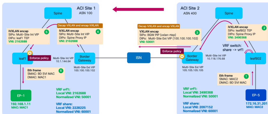
Figure 362. ACI Site 2 VRF share to ACI Site 1 VRF vrf1, ingress leaf performs VRF switch
