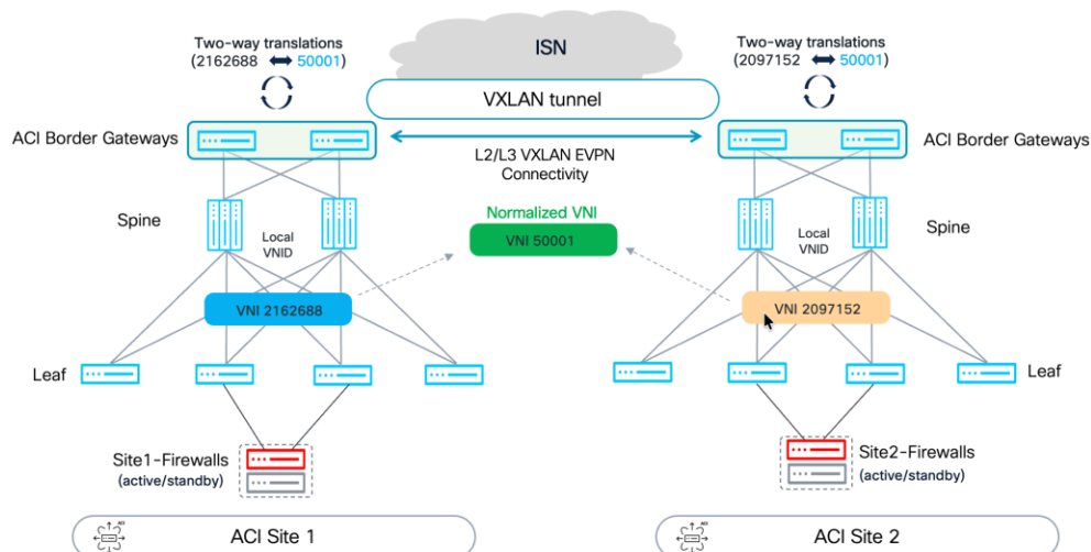
Figure 442. Firewall Insertion Topology
