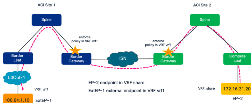
Figure 440. Local endpoint in ACI Site 2 VRF share to external endpoint in ACI Site 1 VRF vrf1
