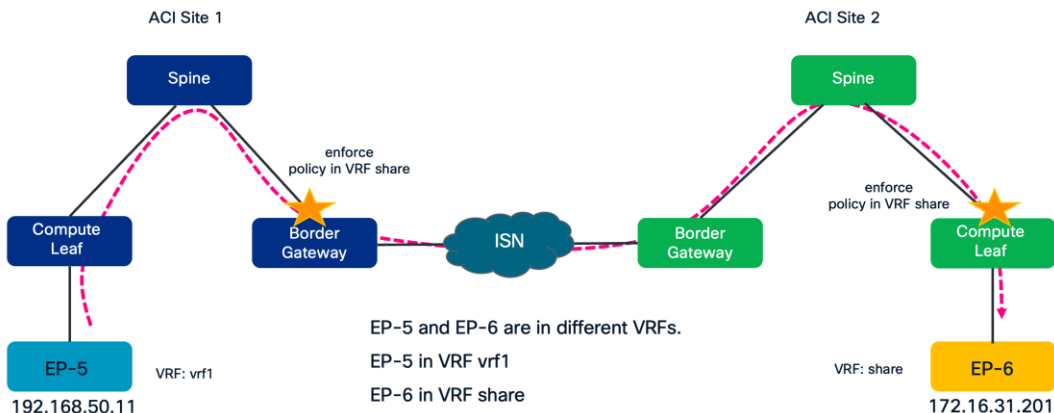
Figure 410. Policy enforcement VRF vrf1 to VRF share, from ACI Site 1 to ACI Site 2
