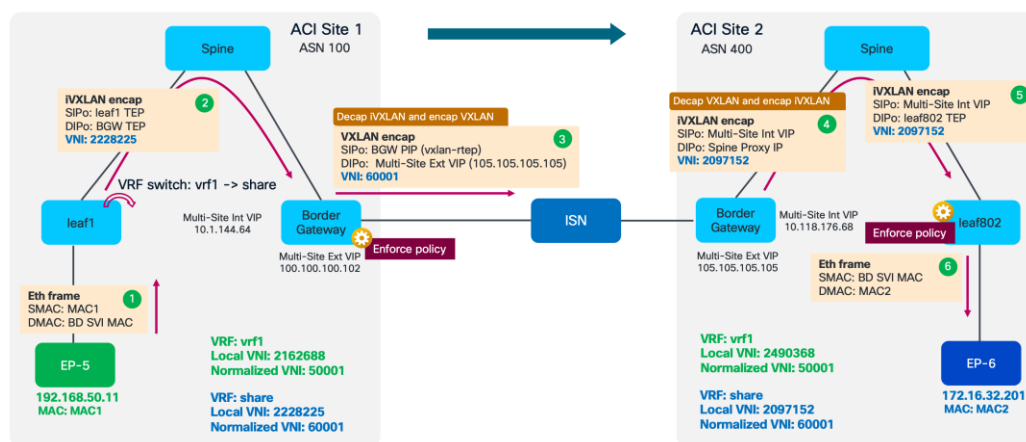
Figure 405. ACI Site 1 VRF vrf1 to ACI Site 2 VRF share, ingress leaf performs VRF switch
