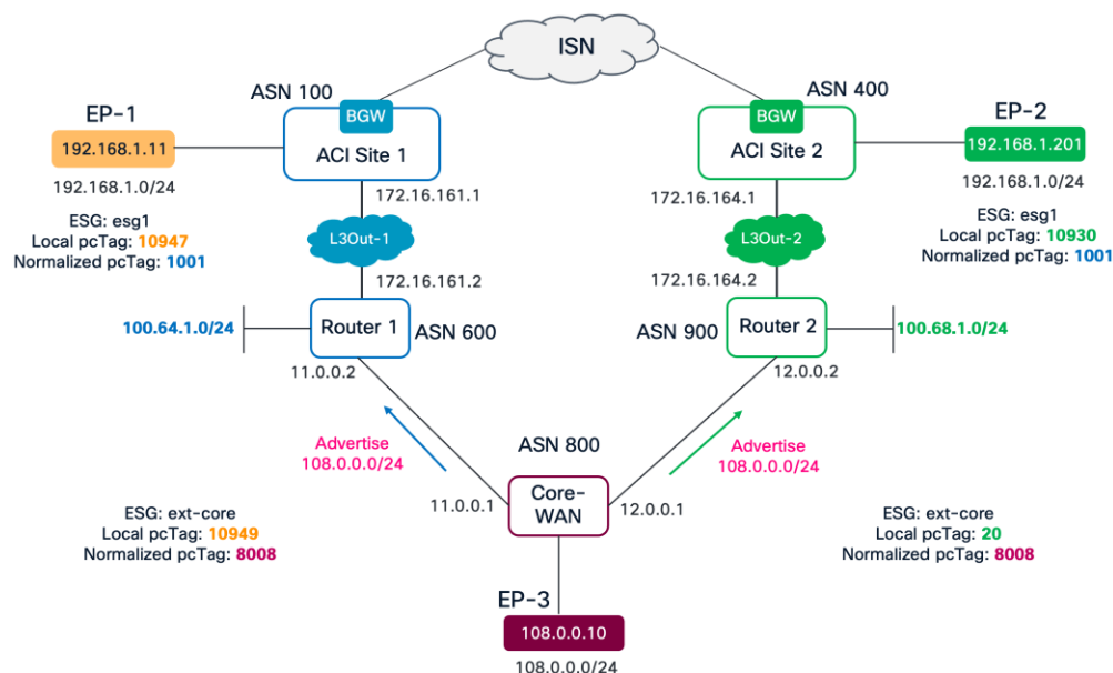
Figure 296. Overlapping Prefix multiple L3Outs
