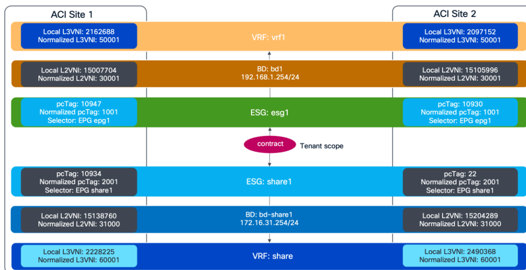
Figure 318. Shared Service use case
