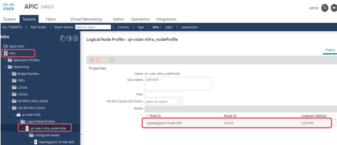
Figure 33. ACI Site 2 Border Gateway qt-bgw805 Logical Node Profile
