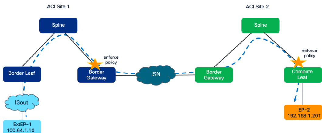
Figure 238. ACI Site 1 external endpoint to ACI Site 2 internal endpoint
