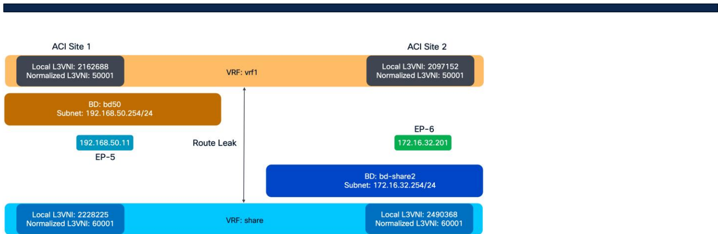
Figure 390. Route Leak diagram
