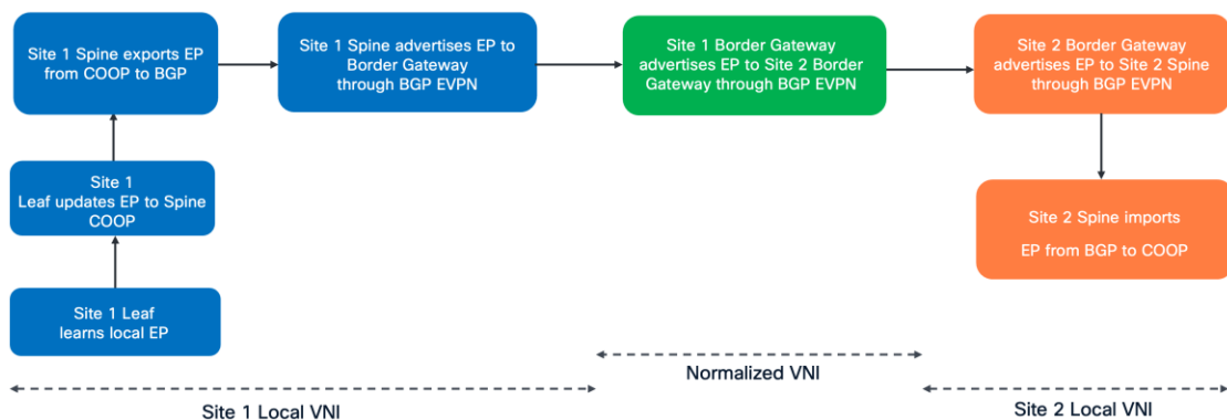
Figure 95. Control Plane across sites
