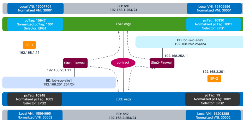
Figure 443. Firewall Insertion Logical Diagram
