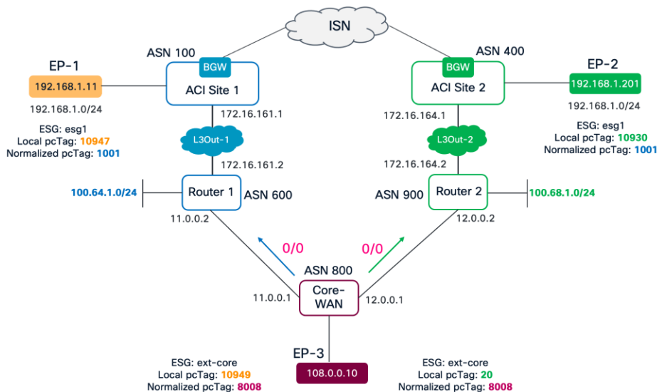
Figure 315. External router advertises default route to both ACI sites
