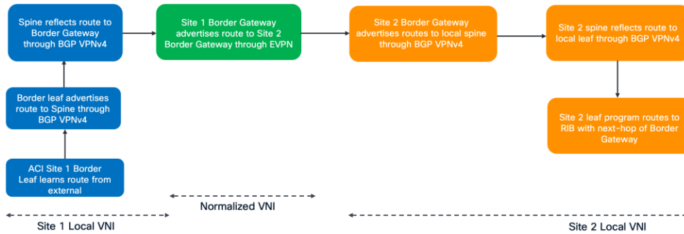
Figure 220. EVPN Type-5 update from ACI Site 1 to Site 2
