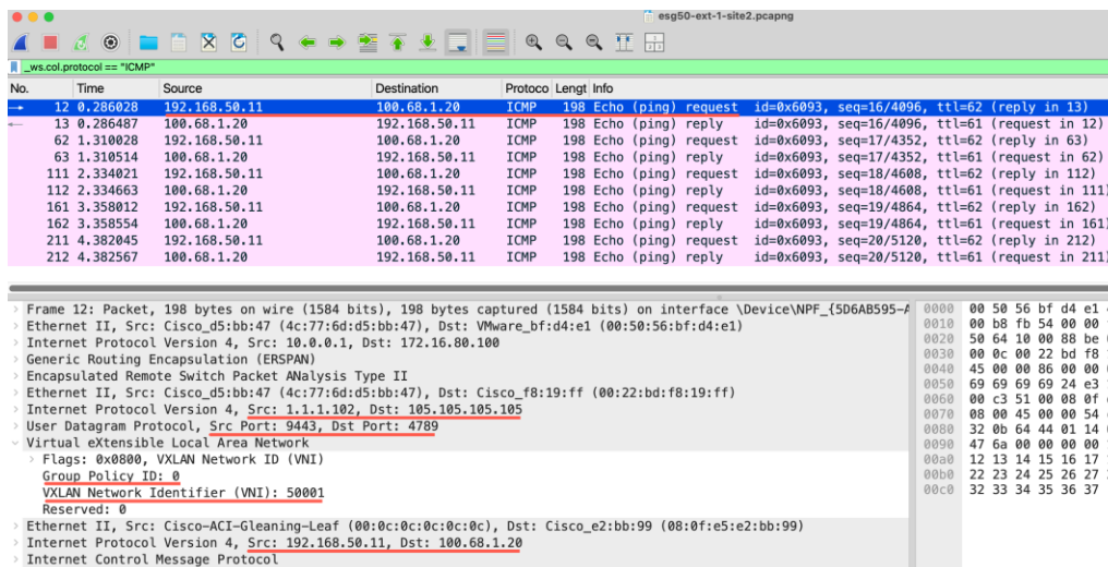
Figure 263. ICMP request from EP-1 (192.168.50.11) to ExtEP-2 (100.68.1.20)
