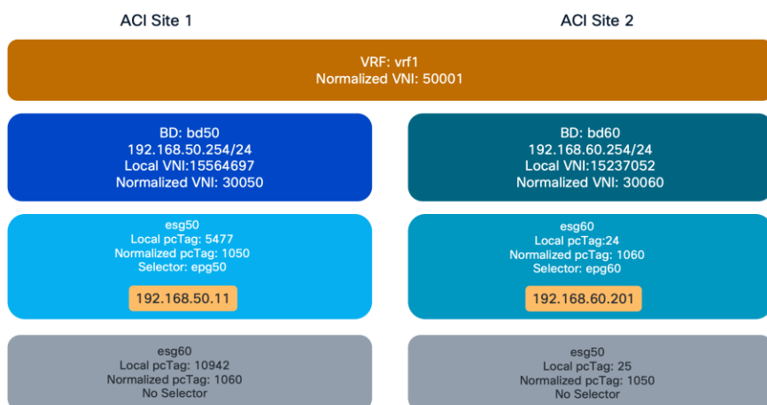
Figure 187. Non-stretch BD multiple ESGs
