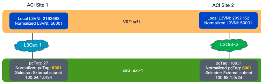
Figure 289. ESG ext-1 with normalized pcTag 8001
