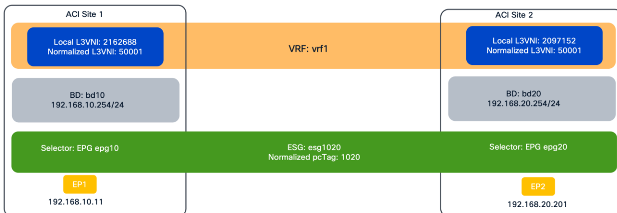
Figure 131. Inter-Subnet Communication Non-Stretched BDs Single ESG
