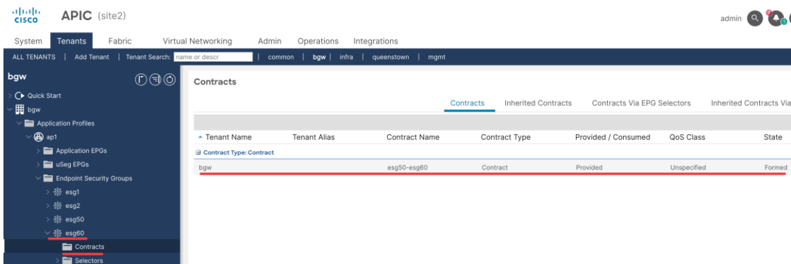
Figure 186. ACI Site 2 esg60 contract provider
