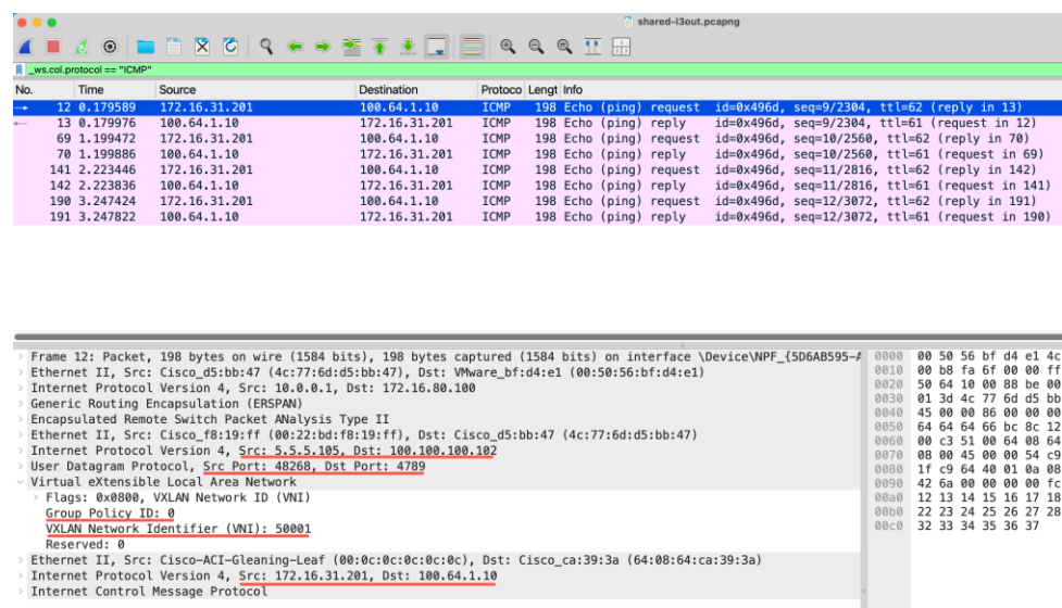
Figure 438. ICMP request from EP-2 (172.16.31.201) to ExtEP-1 (100.64.1.10)
