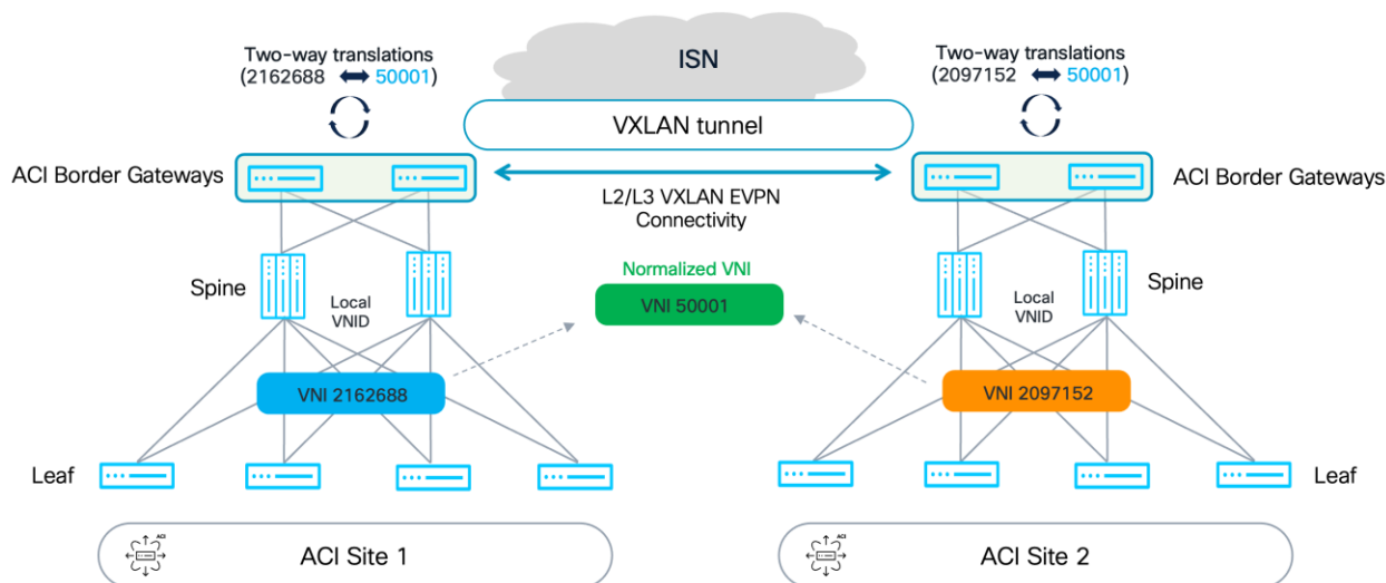
Figure 5. Normalized VNI two-way translations
