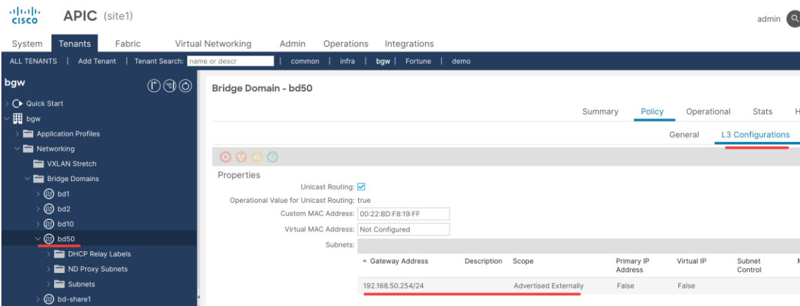
Figure 167. ACI Site 1 bd50 L3 Configurations
