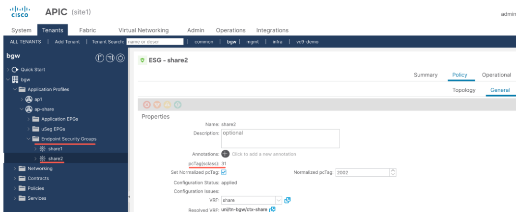
Figure 398. ACI Site 1 ESG share2 local pcTag
