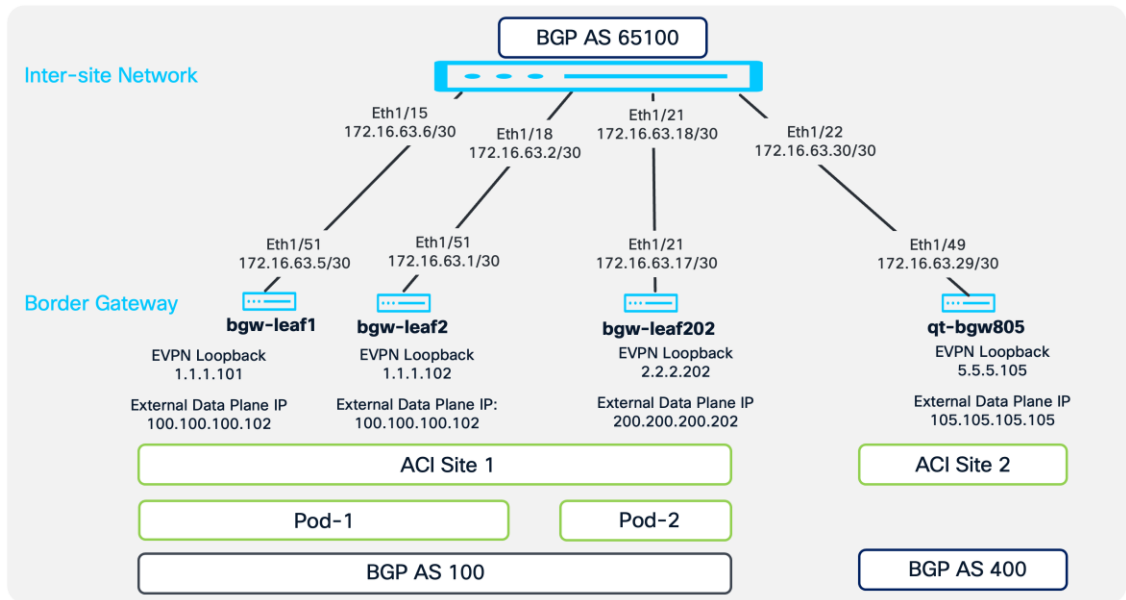
Figure 2. IP Addressing and BGP AS numbers
