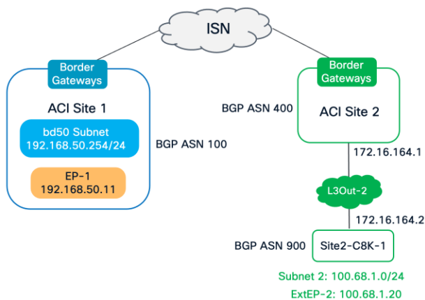
Figure 258. North-South Communication Across Sites with non-stretched (local) BD
