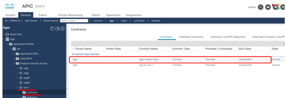
Figure 428. ACI Site 1 ESG ext-1 contract provider
