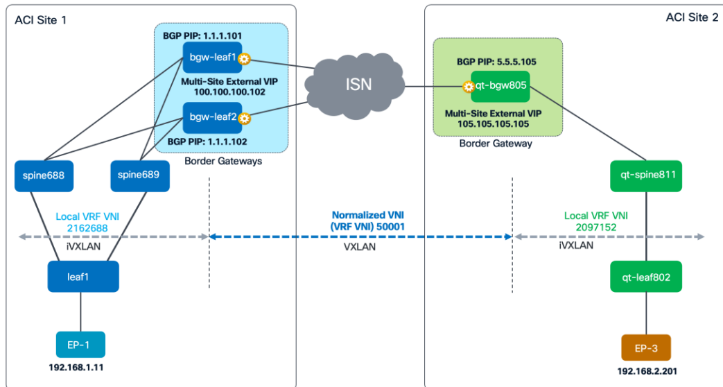
Figure 126. Data plane Routed Communication across sites
