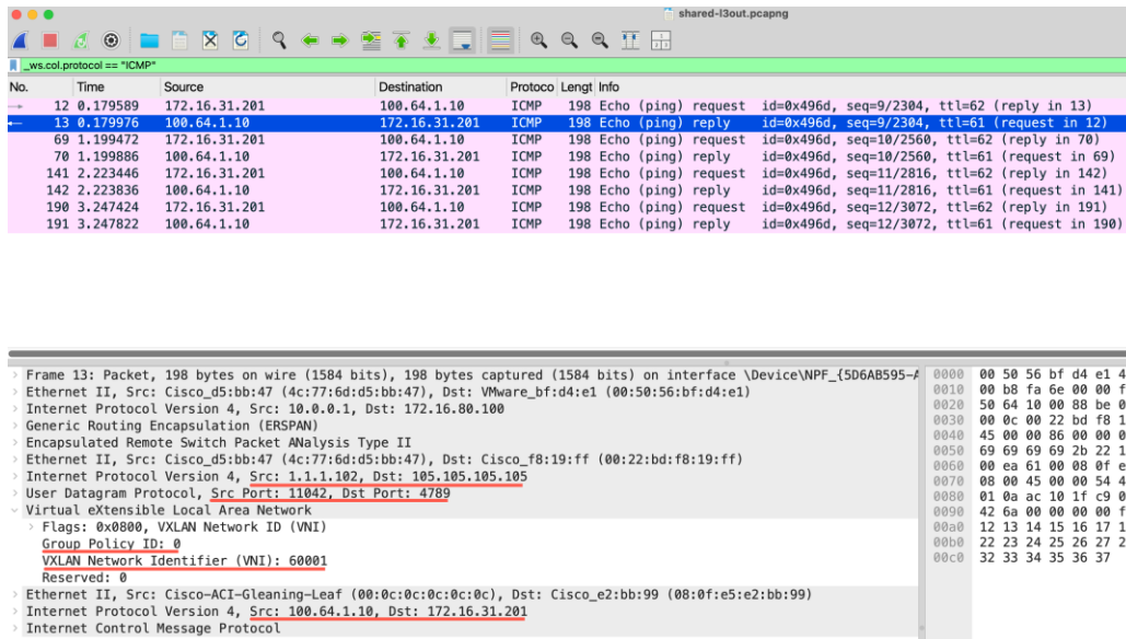
Figure 439. ICMP reply from ExtEP-1 (100.64.1.10) to EP-2 (172.16.31.201)
