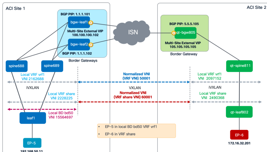
Figure 407. Data plane Inter-VRF Communication (Shared Services) with Non-stretched BDs
