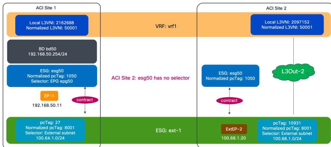
Figure 239. North-South Communication across ACI sites with non-stretched (local) BD
