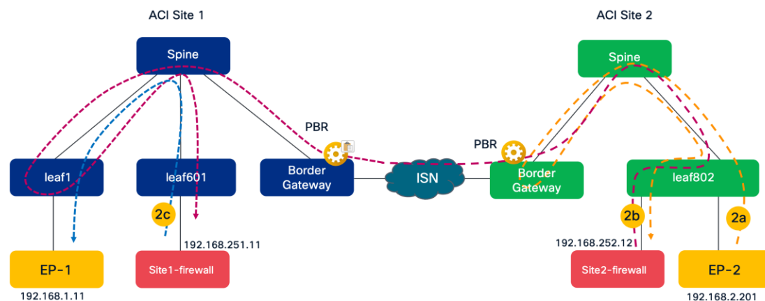
Figure 445. Returning flow from ACI Site 2 esg1 endpoint to ACI Site 1 esg2 endpoint
