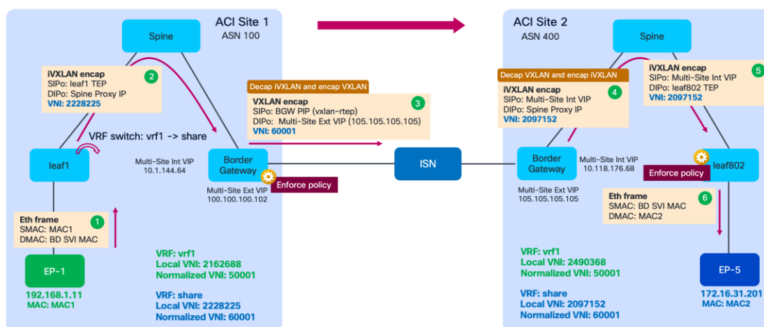
Figure 361. ACI Site 1 VRF vrf1 to ACI Site 2 VRF share, ingress leaf performs VRF switch
