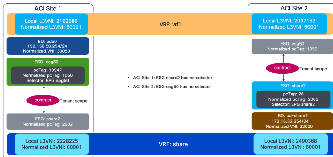
Figure 368. Shared Service with Non-stretched BDs
