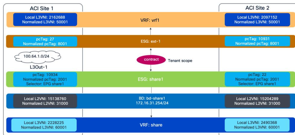
Figure 412. Shared L3Out across ACI Sites
