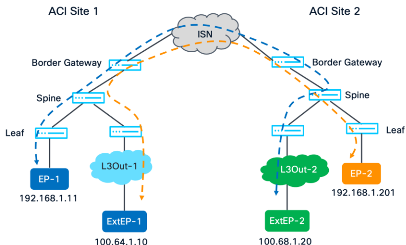
Figure 205. North-South Communication across ACI Sites
