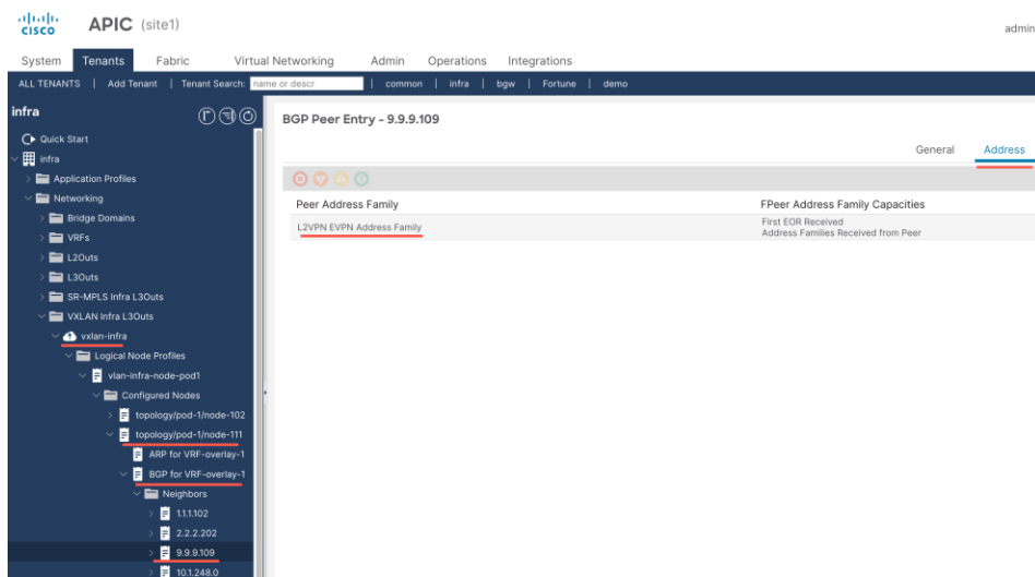
Figure 52. L2VPN EVPN Address Family
