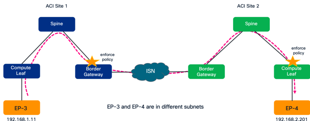
Figure 129. Inter-subnet communication policy enforcement Site 1 to Site 2
