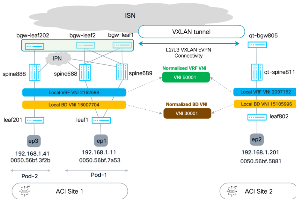
Figure 96. Control Plane verification topology
