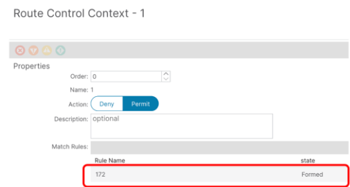
Figure 423. Route Context
