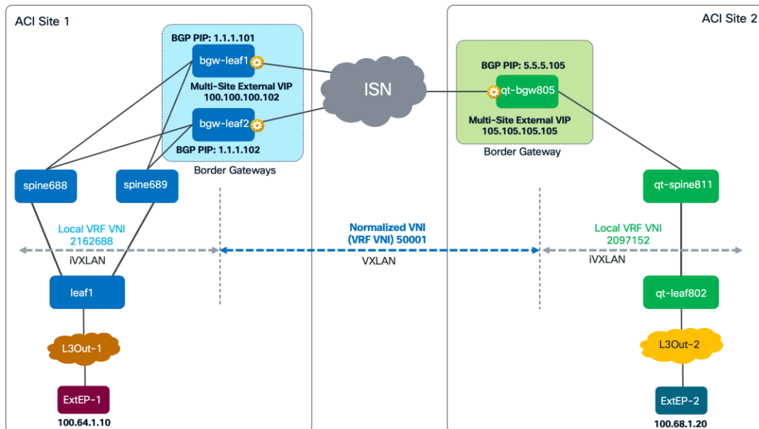
Figure 292. Transit Routing
