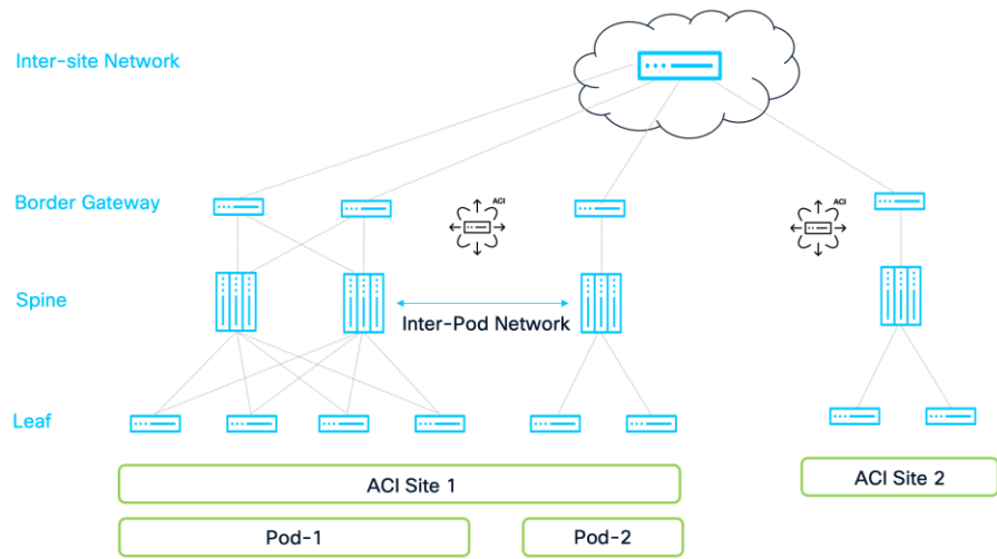
Figure 1. Reference physical topology
