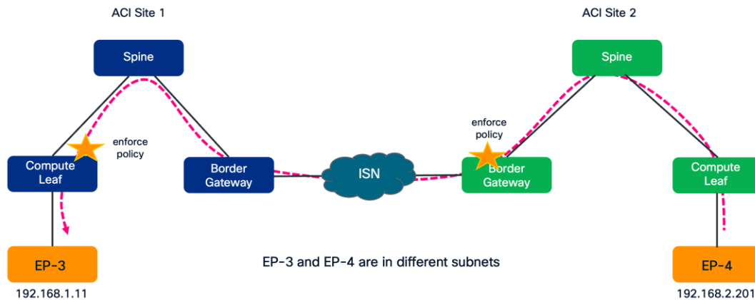
Figure 130. Inter-subnet communication policy enforcement Site 2 to Site 1
