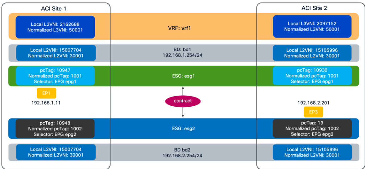
Figure 113. Inter-Subnet Communication
