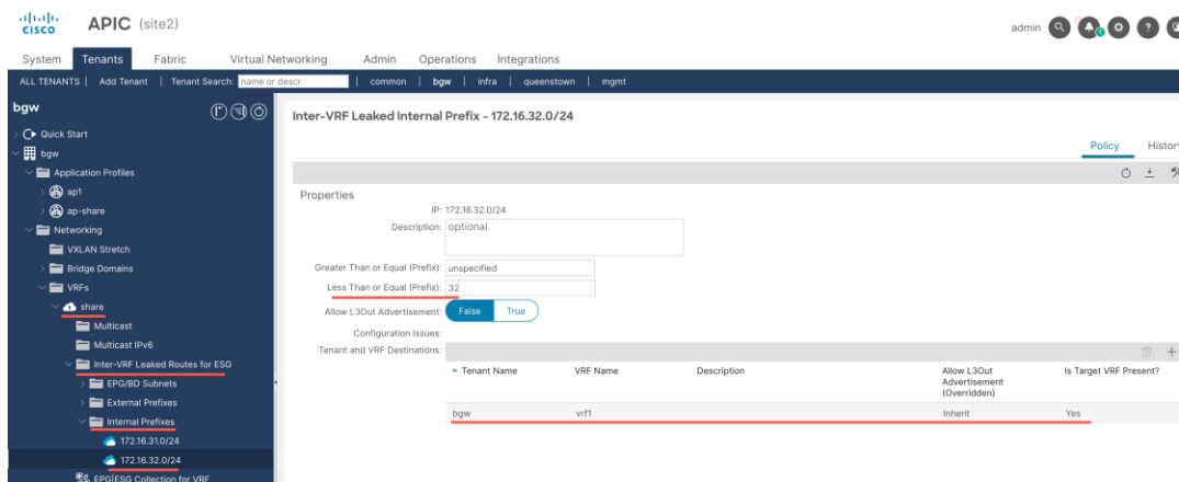
Figure 389. ACI Site 2 leak prefix 172.16.32.0/24 from VRF share to VRF vrf1
