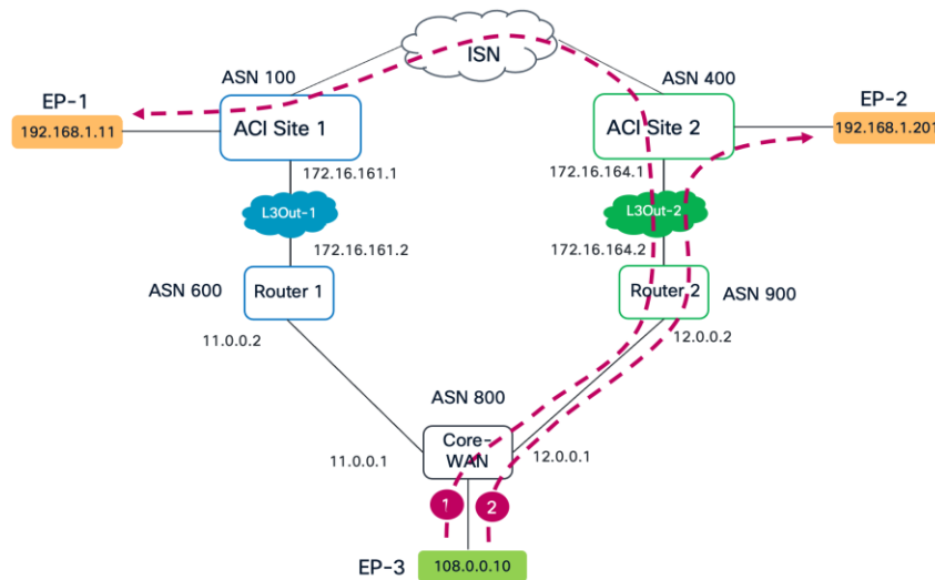
Figure 308. Non-optimal incoming flow
