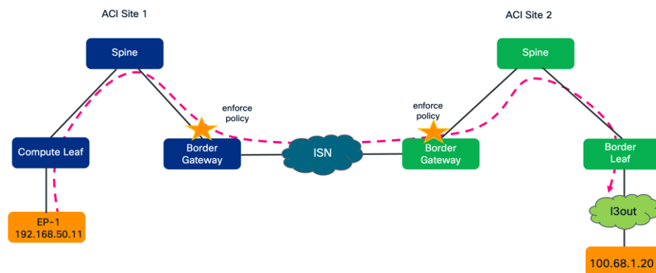
Figure 265. ACI Site 1 internal endpoint to ACI Site 2 external endpoint
