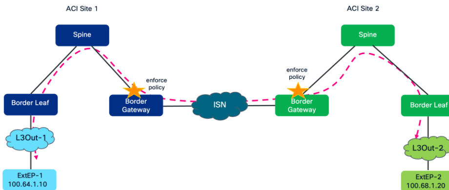
Figure 295. Policy enforcement Transit Routing across sites
