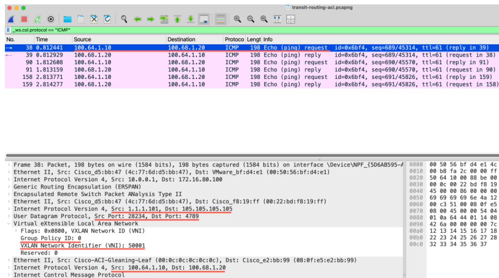
Figure 293. ICMP request from ExtEP-1 (100.64.1.10) to ExtEP-2 (100.68.1.20)
