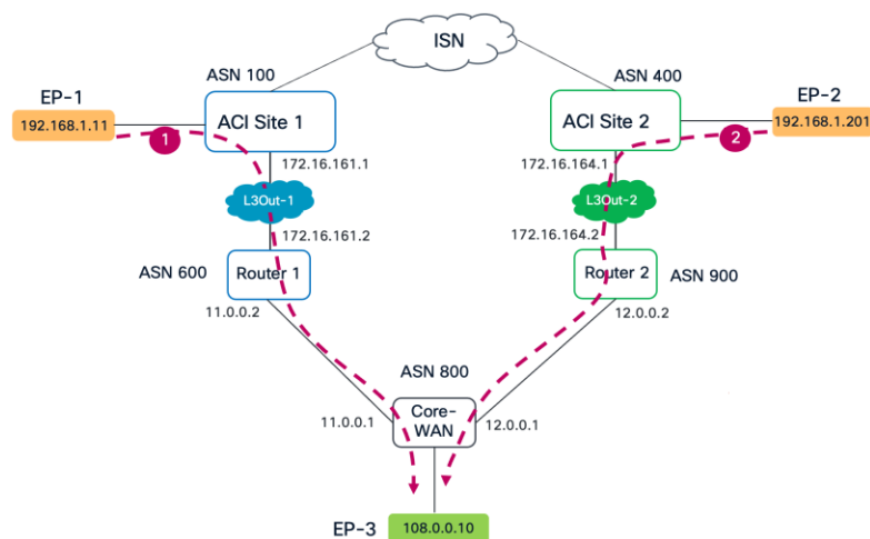
Figure 305. Outbound flow from ACI Site connected endpoint to external
