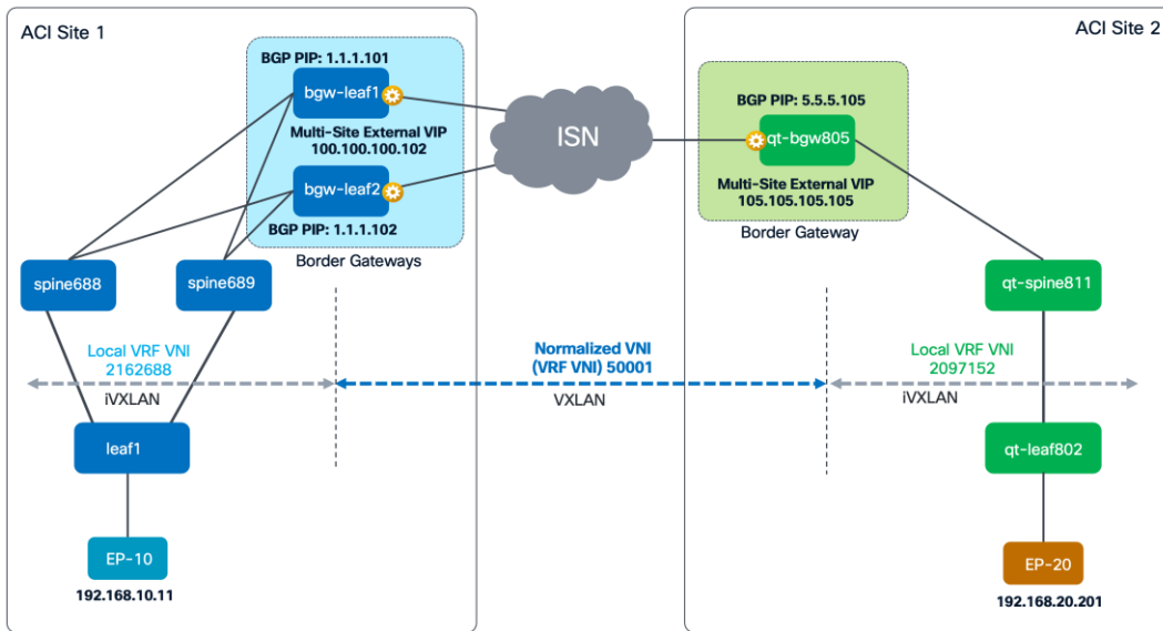
Figure 161. Data plane Inter-Subnet Communication with Non-stretched BDs and Single ESG
