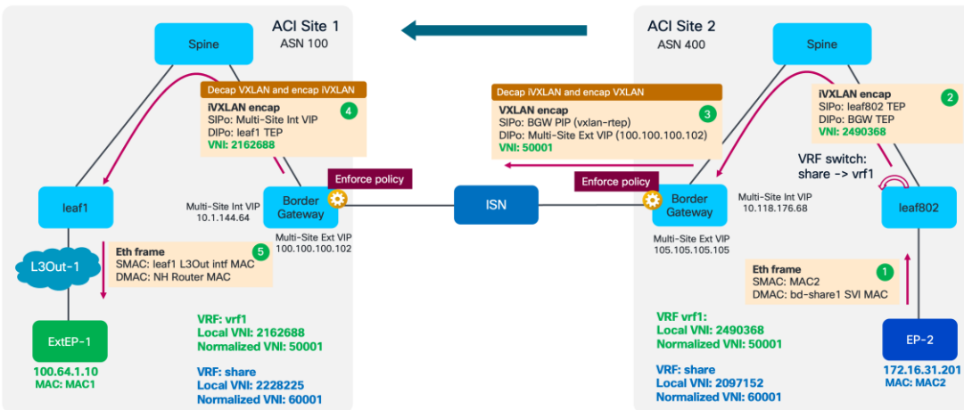
Figure 435. ACI Site 2 VRF share to ACI Site 1 VRF vrf1 L3Out, ingress leaf performs VRF switch
