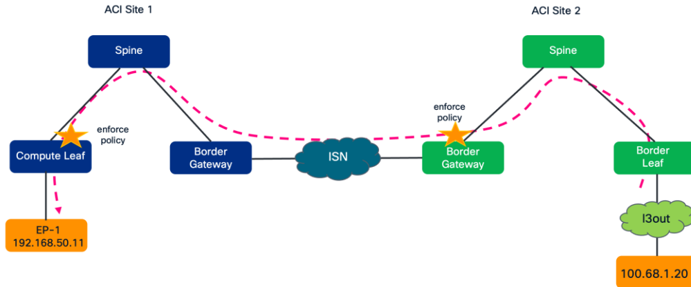
Figure 266. ACI Site 2 external endpoint to ACI Site 1 internal endpoint
