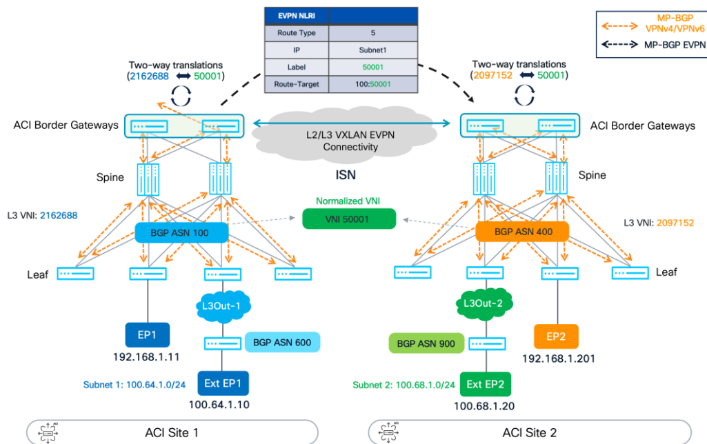
Figure 219. EVPN Type 5 Route exchange across ACI Sites
