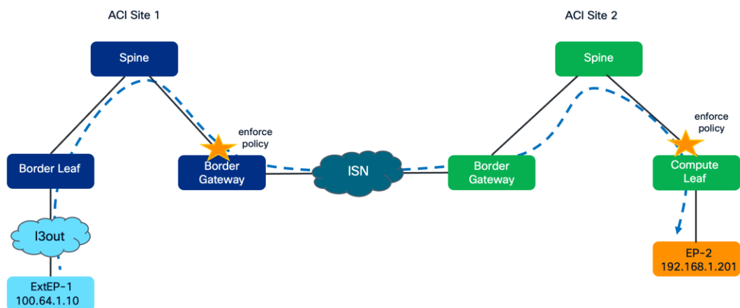
Figure 238. ACI Site 1 external endpoint to ACI Site 2 internal endpoint
