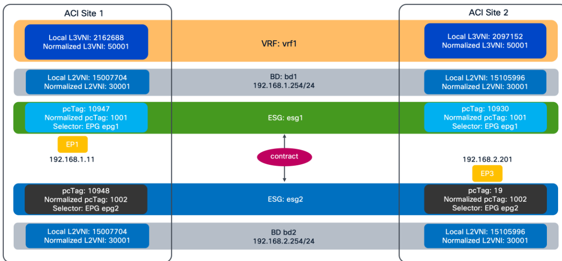
Figure 113. Inter-Subnet Communication
