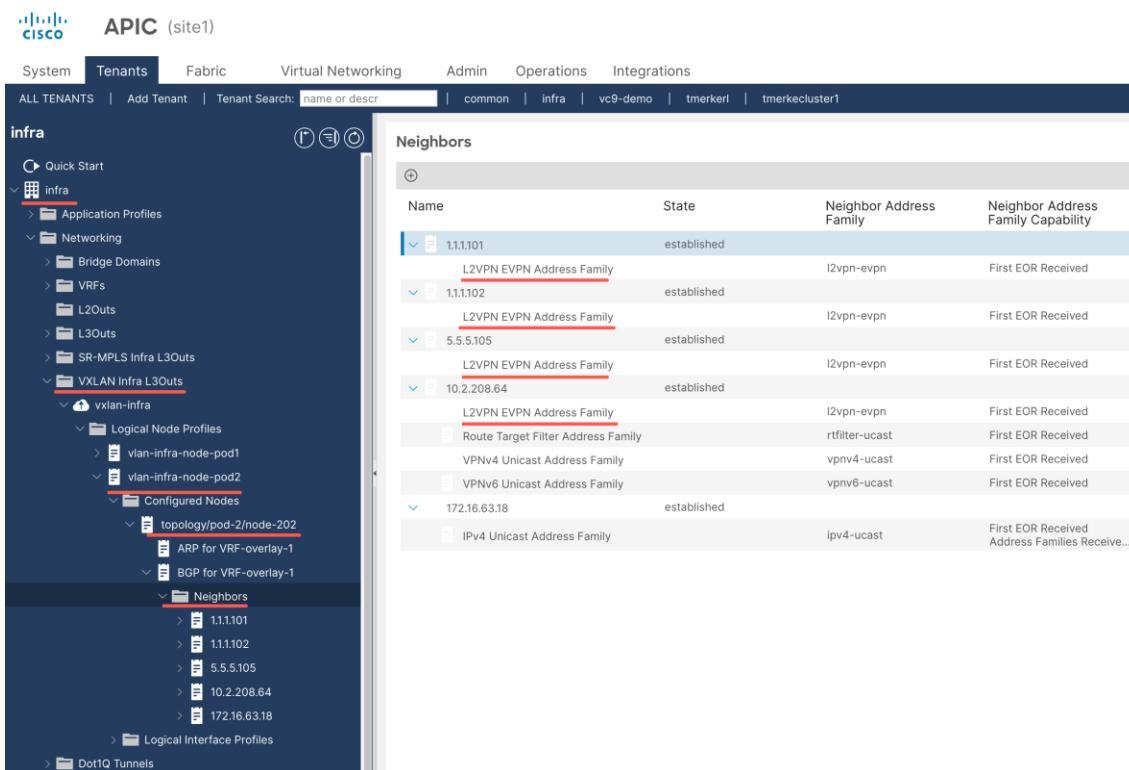
Figure 41. ACI Site 1 Border Gateway bgw-leaf202 BGP EVPN neighbors
