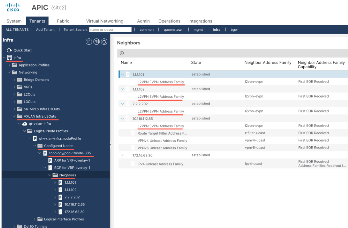
Figure 42. ACI Site 2 Border Gateway qt-bgw805 BGP EVPN neighbors
