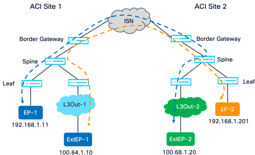
Figure 205. North-South Communication across ACI Sites
