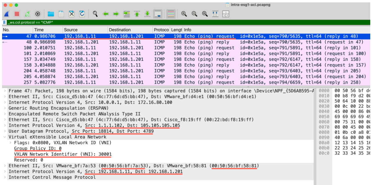
Figure 110. ICMP request from EP-1 (192.168.1.11) to EP-2 (192.168.1.201)
