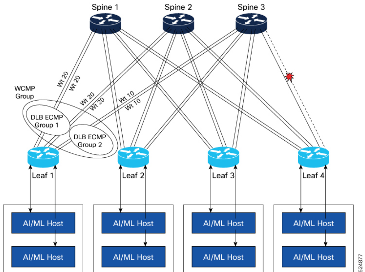
Figure 2: Hierarchical WCMP
