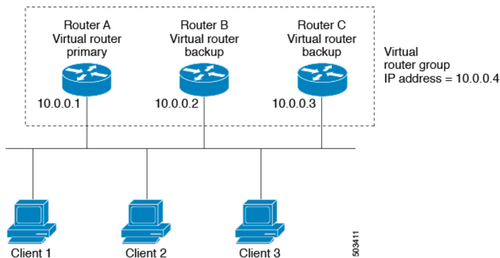
Figure 47: Basic VRRP Topology
