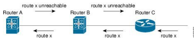
Figure 37: RIPng with Split Horizon Poison Reverse
