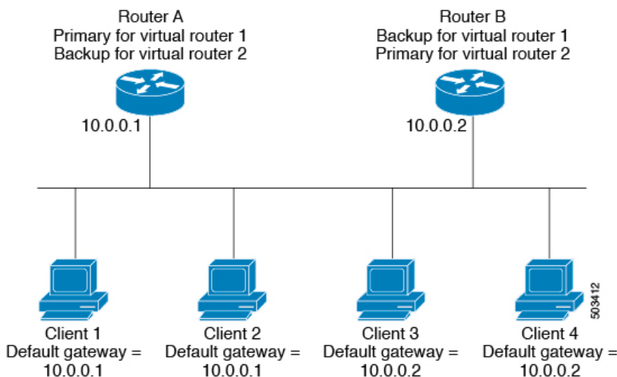
Figure 48: Load Sharing and Redundancy VRRP Topology
