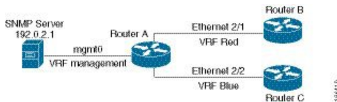
Figure 41: Service VRF Reachability Filtering
