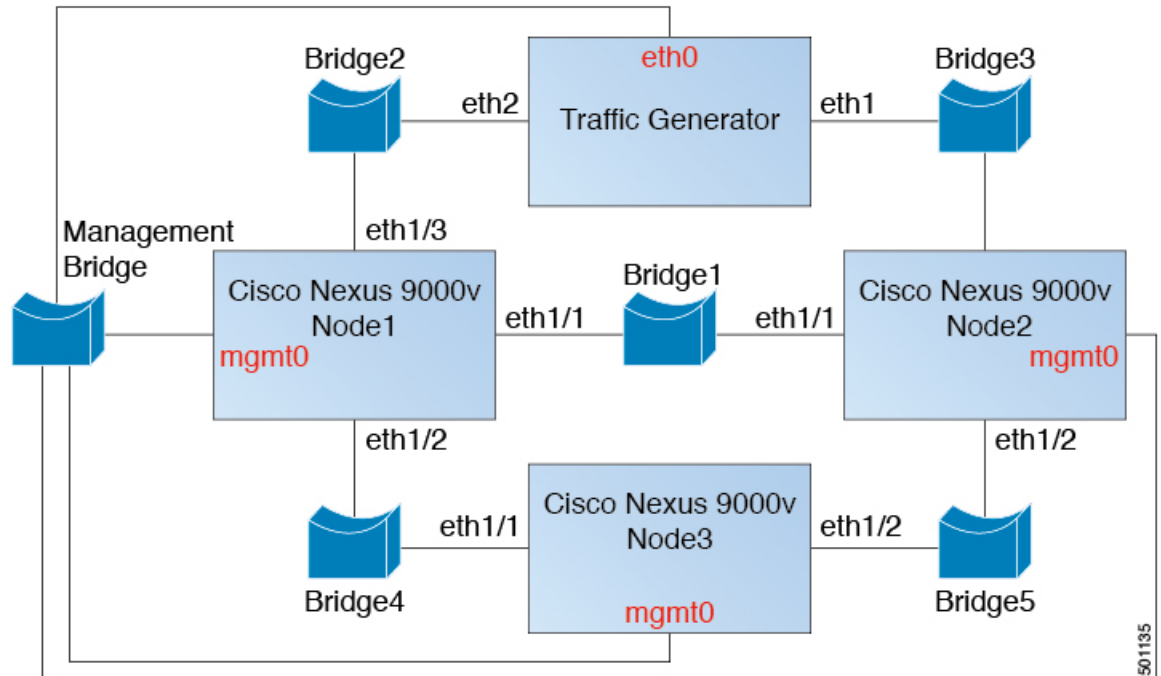
Figure 1: Interconnecting Cisco Nexus 9000v Platforms through EXSi
