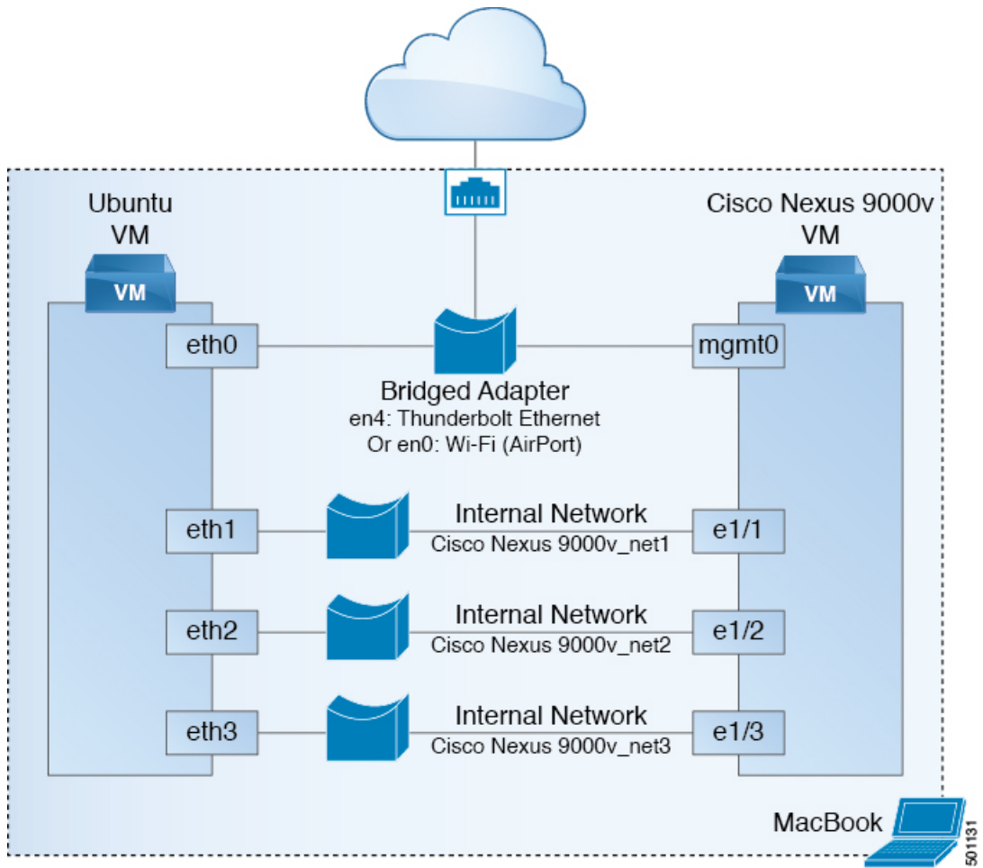
Figure 2: Interconnecting Cisco Nexus 9000v Platforms through Vagrant VM
