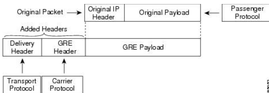
Figure 14: GRE PDU
