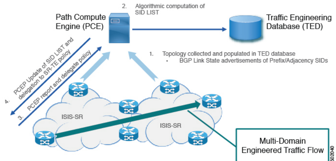
Figure 10: ODN Operation
