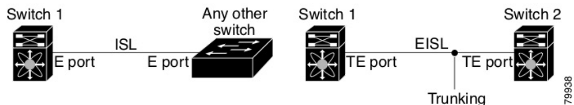
Figure 12: VSAN Trunking Only
