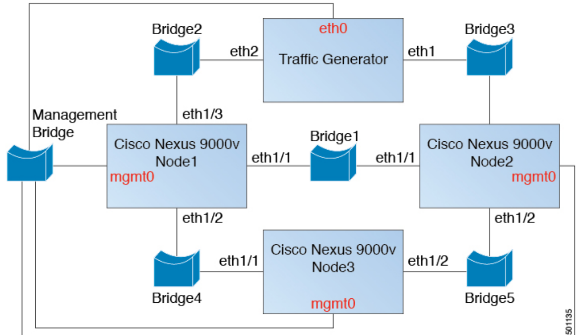
Figure 1: Interconnecting Cisco Nexus 9000v Platforms through ESXi
