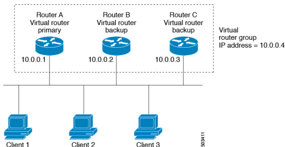
Figure 42: Basic VRRP Topology
