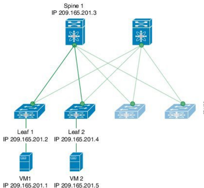
Figure 1: VXLAN Network
