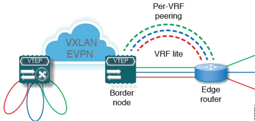
Figure 18: External Layer-3 Connectivity - VRF-lite
