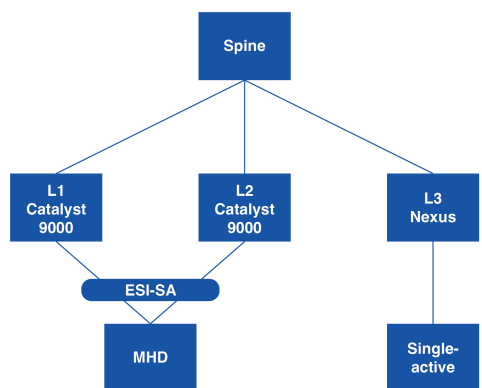
Figure 17: ESI Single-Active Multihoming
