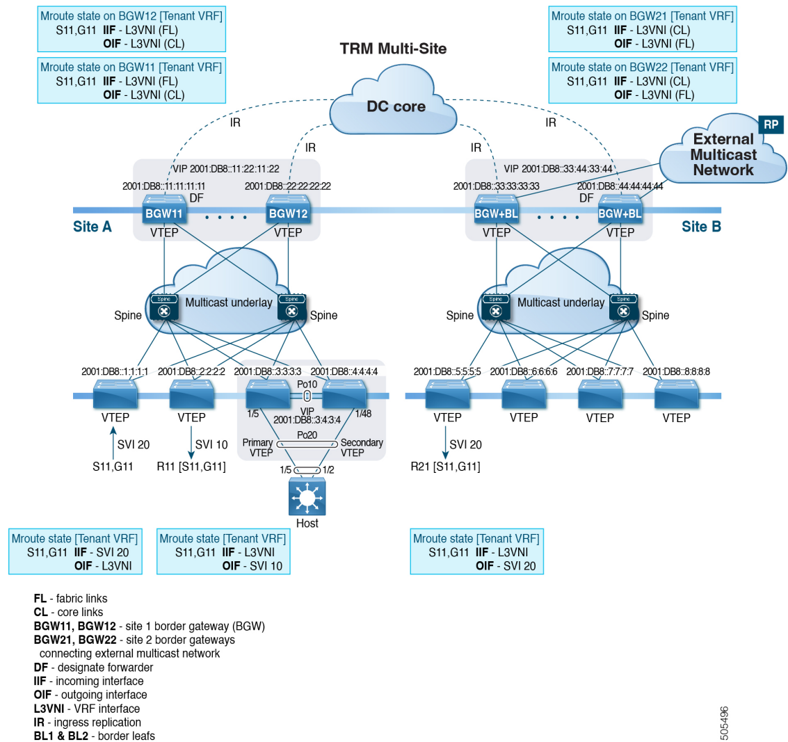
Figure 33: TRM Multi-Site with IPv6 Underlay Topology, BGW External Multicast Connectivity
