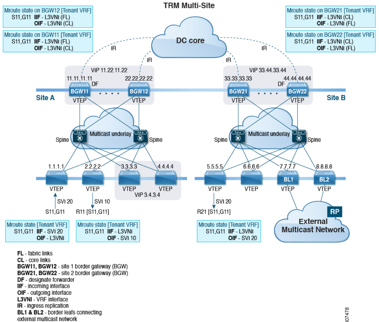
Figure 30: TRM with Multi-Site Topology, BL External Multicast Connectivity
