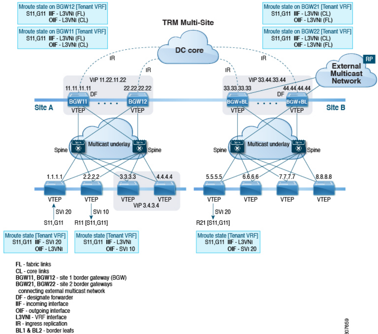
Figure 31: TRM with Multi-Site Topology, BGW External Multicast Connectivity
