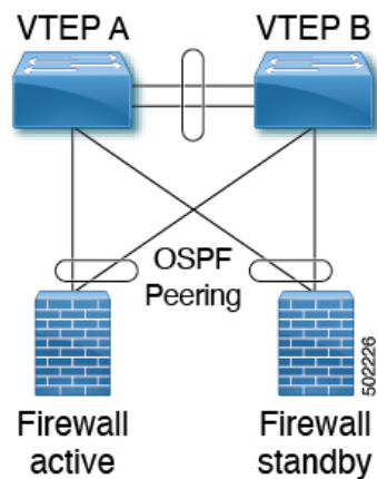
Figure 63: Dual-Attached Firewall with OSPF
