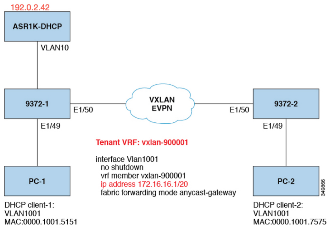
Figure 71: Example Topology
