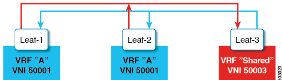
Figure 13: Shared Services VRFs
