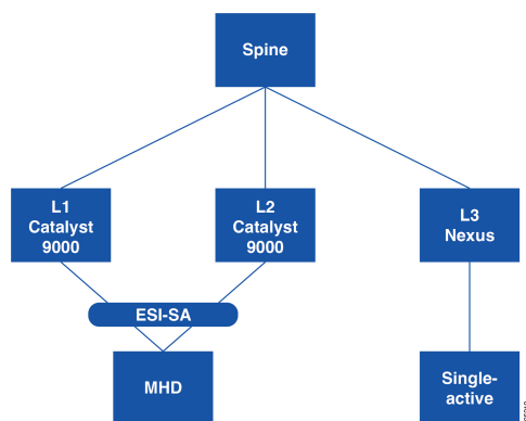
Figure 17: ESI Single-Active Multihoming
