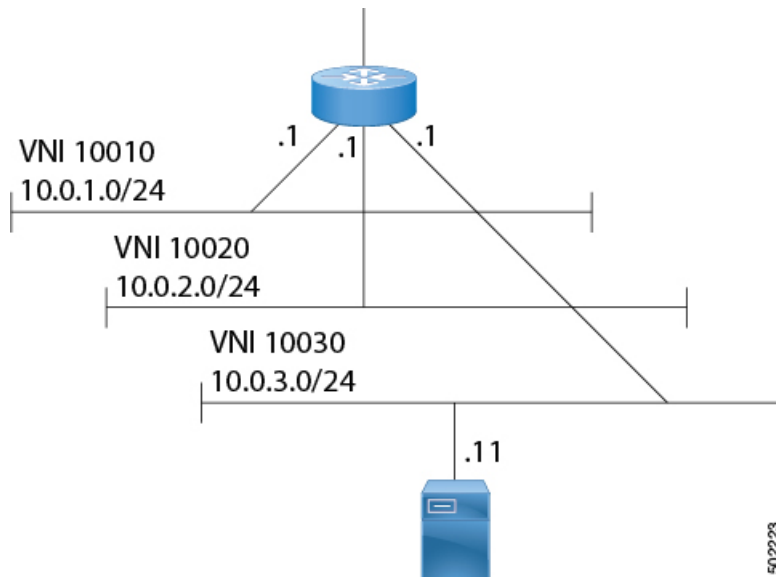
Figure 64: Firewall as Default Gateway with a Layer-2 VXLAN Fabric
