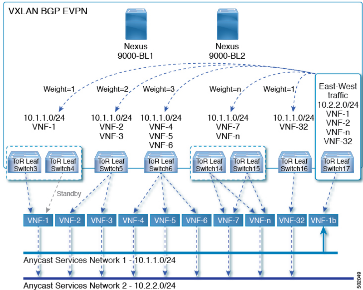
Figure 67: Sample Topology (East-West Traffic)
