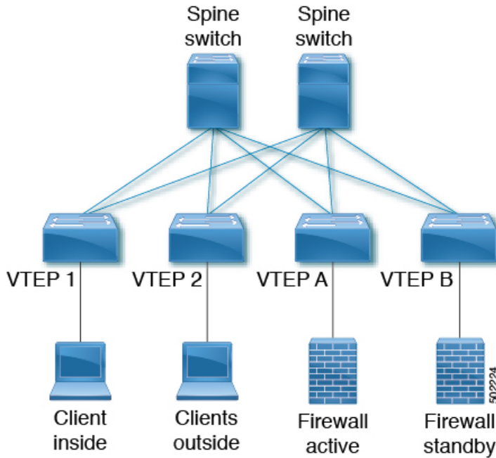
Figure 59: Topology Overview with Firewall Attachment
