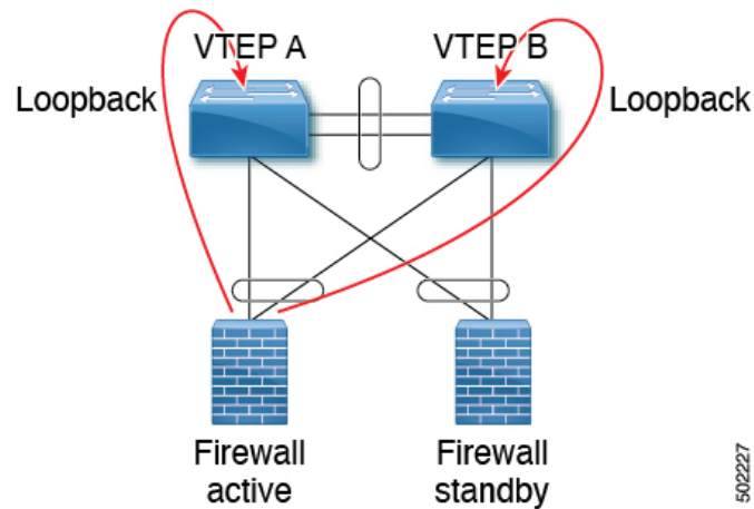
Figure 62: Dual-Attached Firewall with eBGP
