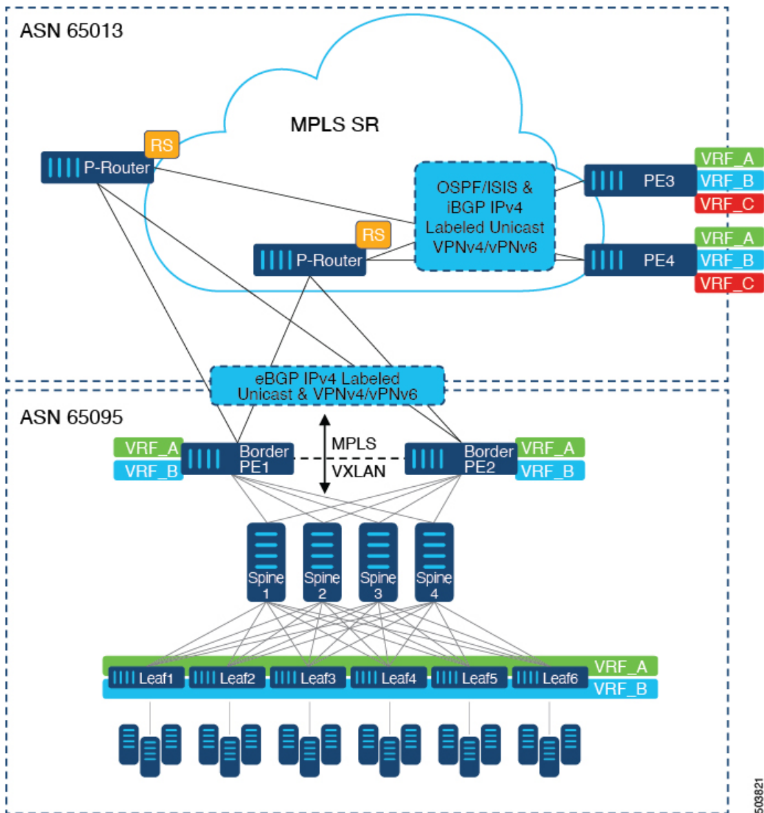
Figure 22: Topology with DC to Core Network Domain Separation
