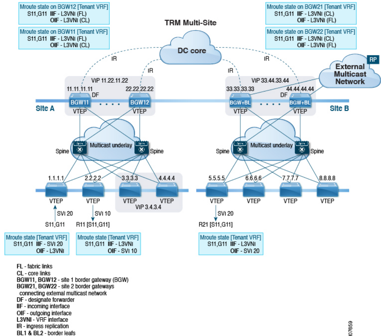
Figure 31: TRM with Multi-Site Topology, BGW External Multicast Connectivity
