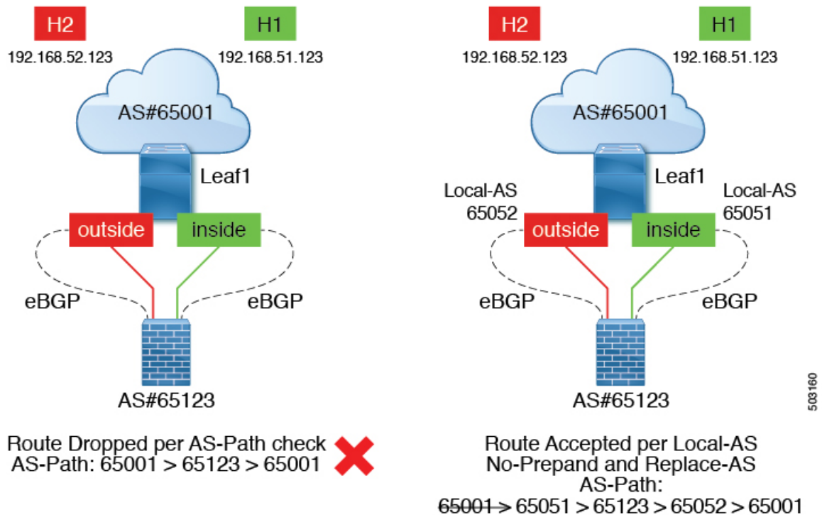
Figure 61: eBGP AS-Path Check
