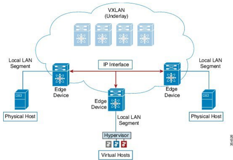
Figure 3: Underlay Overview
