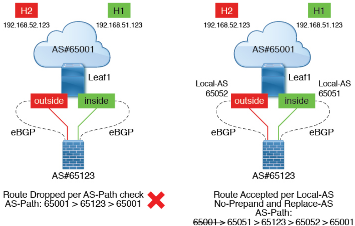
Figure 61: eBGP AS-Path Check
