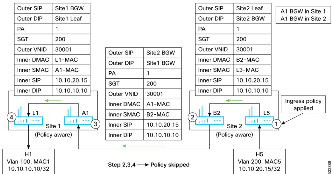
Figure 55: Packet-Flow from Host H5 to Host H1
