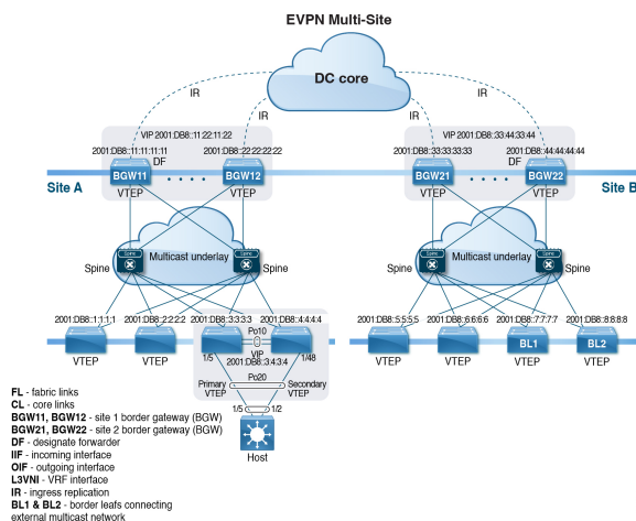
Figure 29: Topology - VXLAN EVPN Multi-Site with IPv6 Underlay
