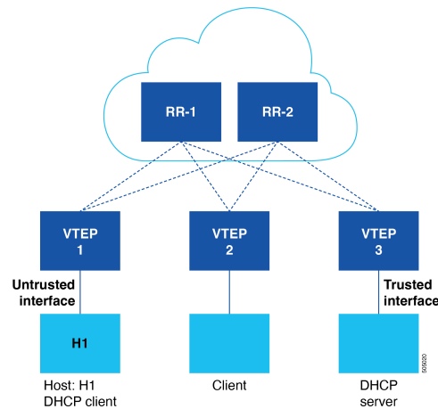
Figure 77: DHCP Snooping on VXLAN
