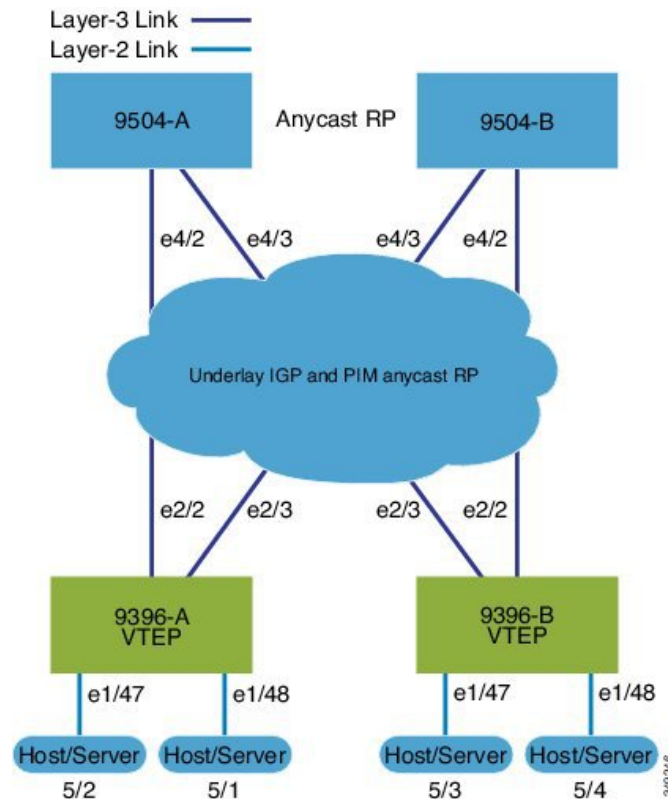
Figure 15: VXLAN BGP EVPN Topology (IBGP)
