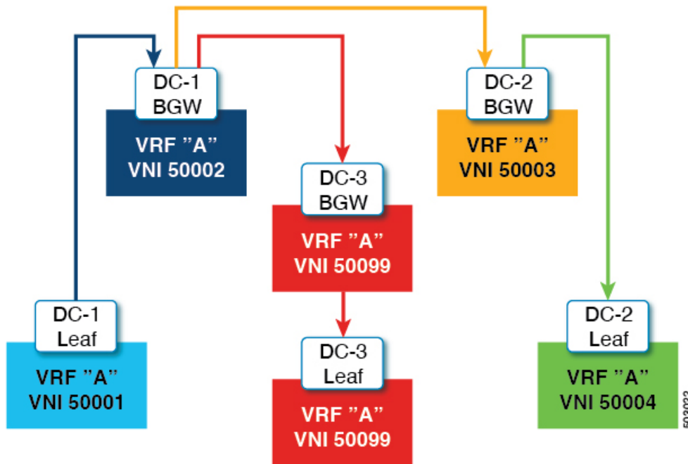
Figure 14: Multi-Site with Asymmetric VNIs
