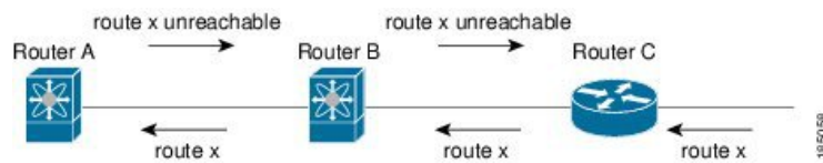
Figure 34: RIPng with Split Horizon Poison Reverse
