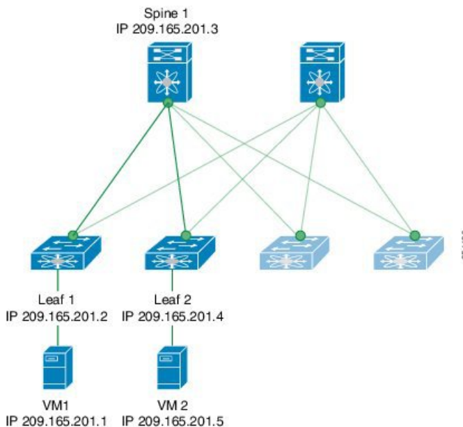
Figure 1: VXLAN Network
