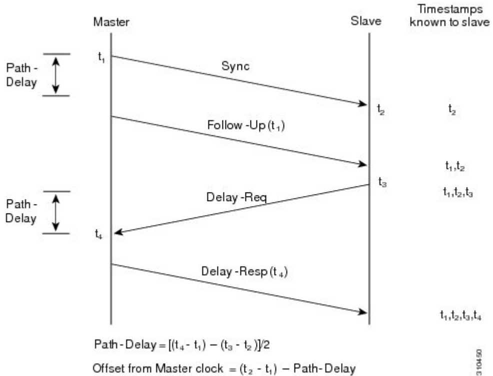
Figure 1: PTP Process
