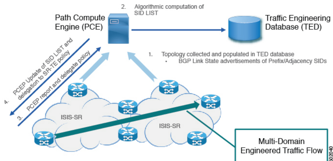
Figure 8: ODN Operation
