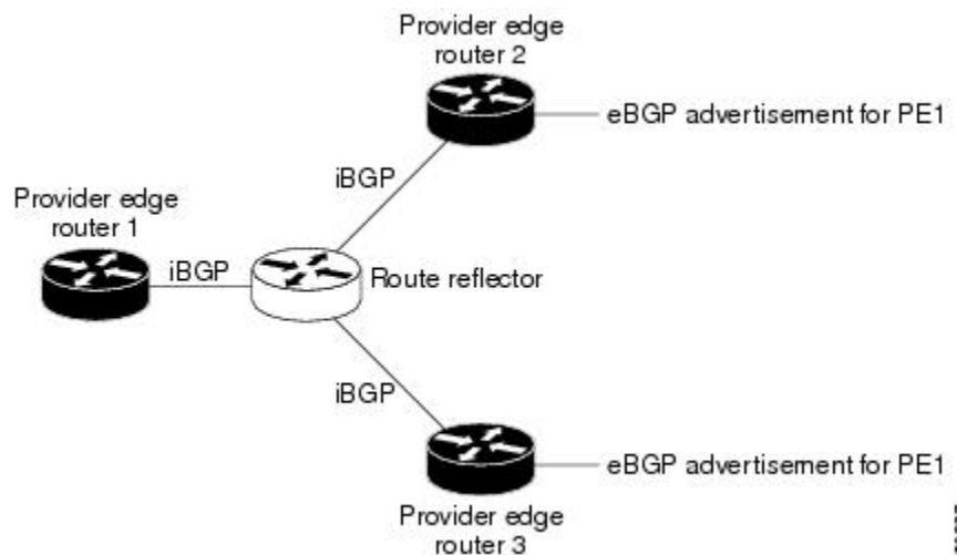
Figure 5: Topology with a Route Reflector
