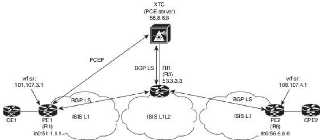
Figure 9: Reference Topology
