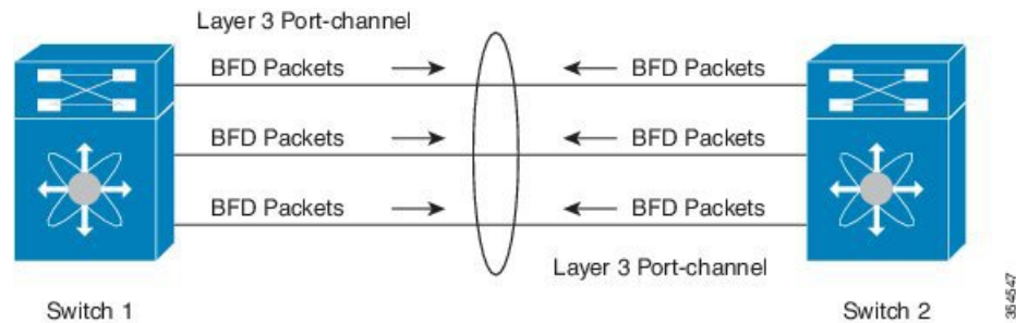
Figure 3: Configuring Micro BFD Session
