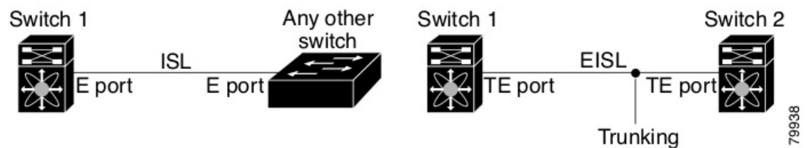
Figure 11: VSAN Trunking Only
