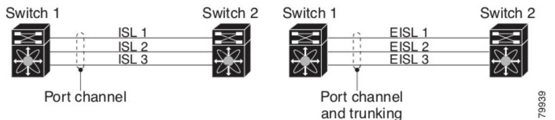
Figure 12: Port Channels and VSAN Trunking
