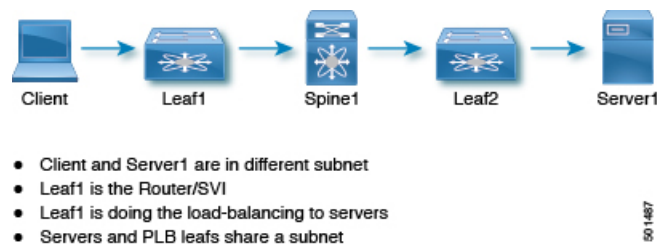
Figure 7: Direct Server Return
