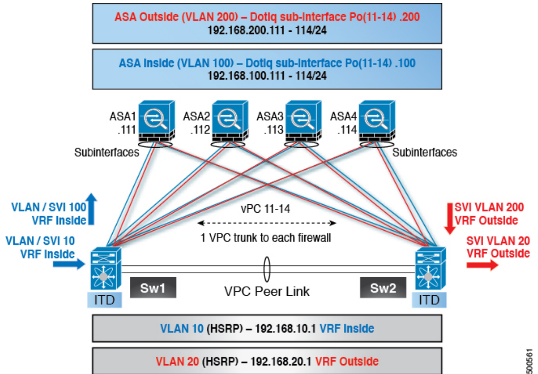
Figure 22: Firewall on a Stick (with vPC) Deployment
