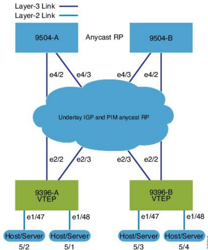
Figure 3: VXLAN BGP EVPN Topology (IBGP)
