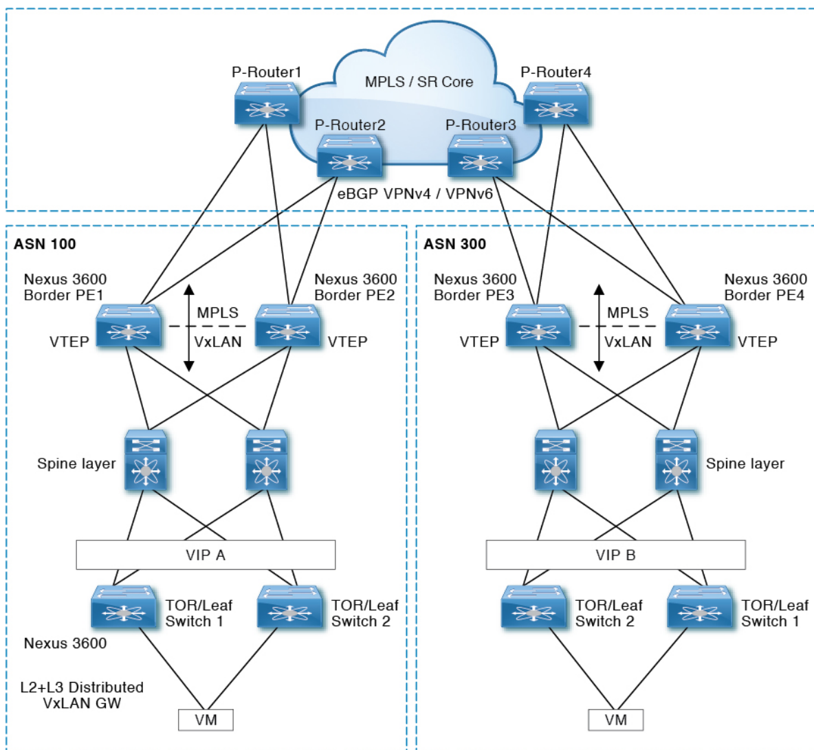
Figure 8: Topology Overview
