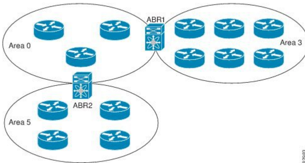
Figure 2: OSPFv2 Areas
