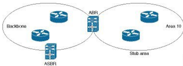
Figure 3: Stub Area
