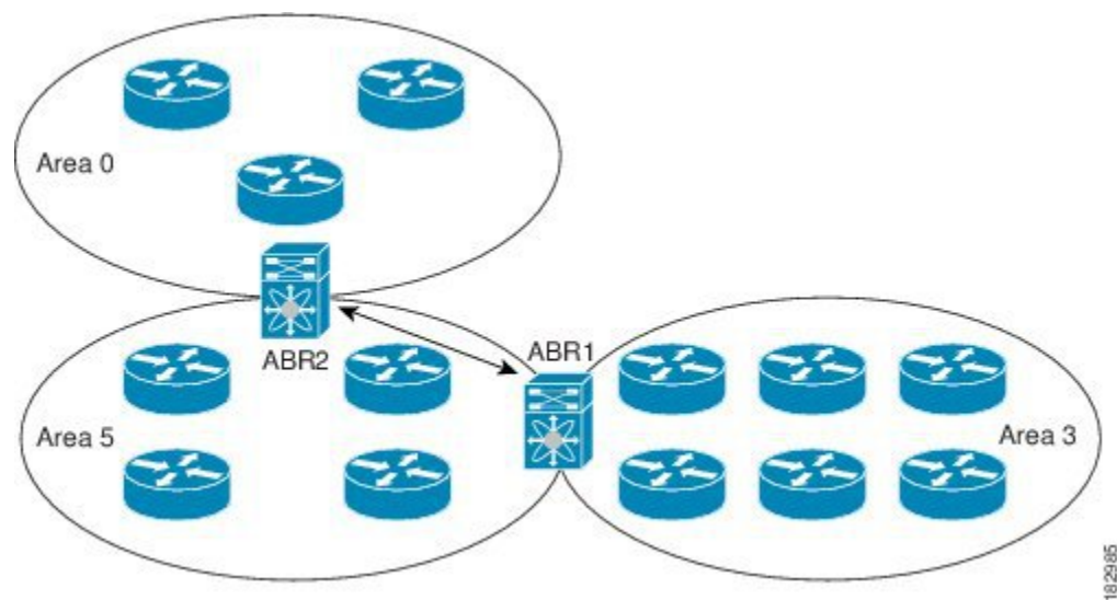
Figure 4: Virtual Links
