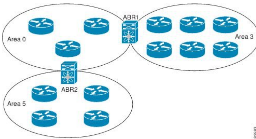
Figure 2: OSPFv2 Areas
