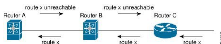
Figure 29: RIP with Split Horizon Poison Reverse
