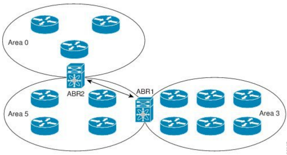
Figure 24: Virtual Links
