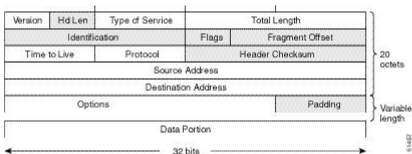
Figure 10: IPv4 Packet Header Format
