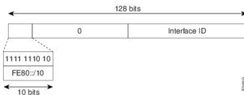
Figure 7: Link-Local Address Format
