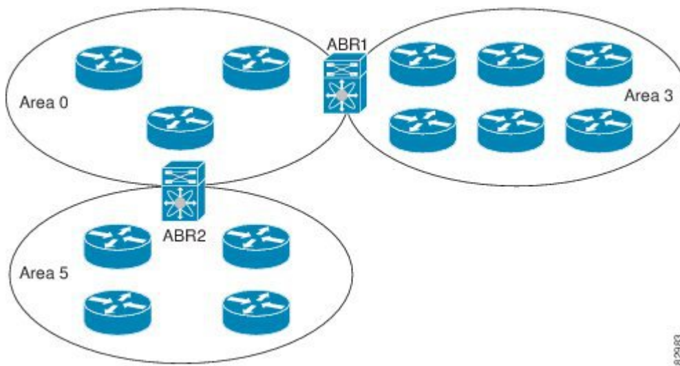
Figure 7: OSPFv2 Areas
