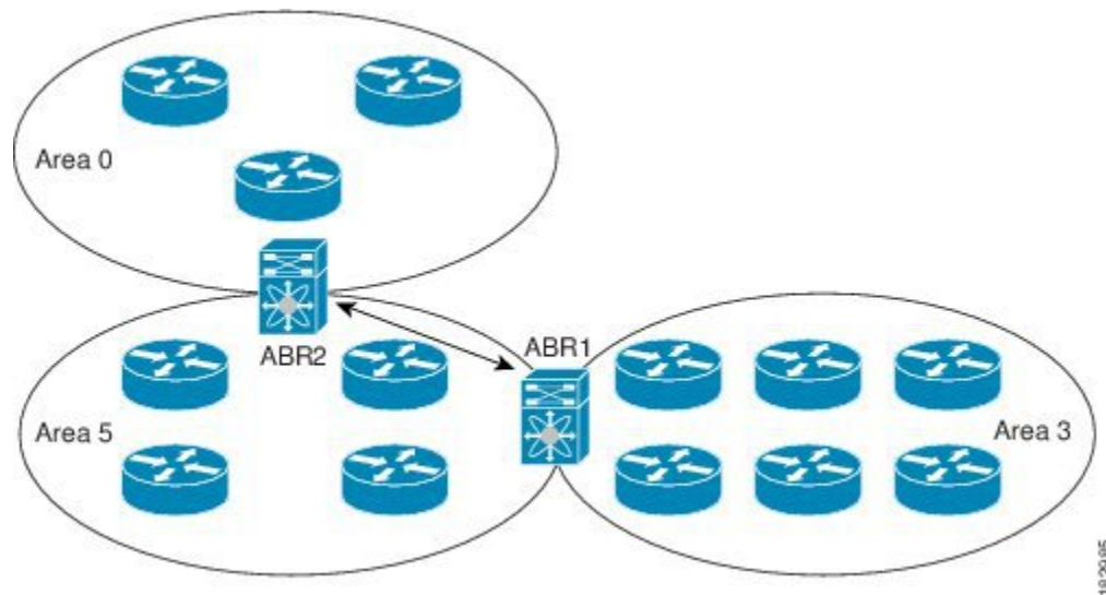
Figure 4: Virtual Links
