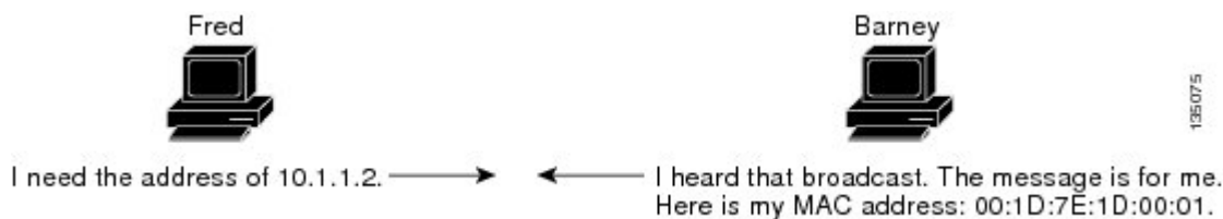
Figure 4: ARP Process
