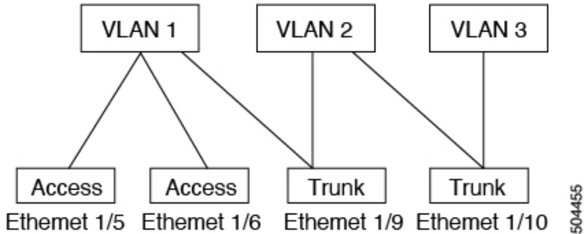
Figure 1: Trunk and Access Ports and VLAN Traffic
