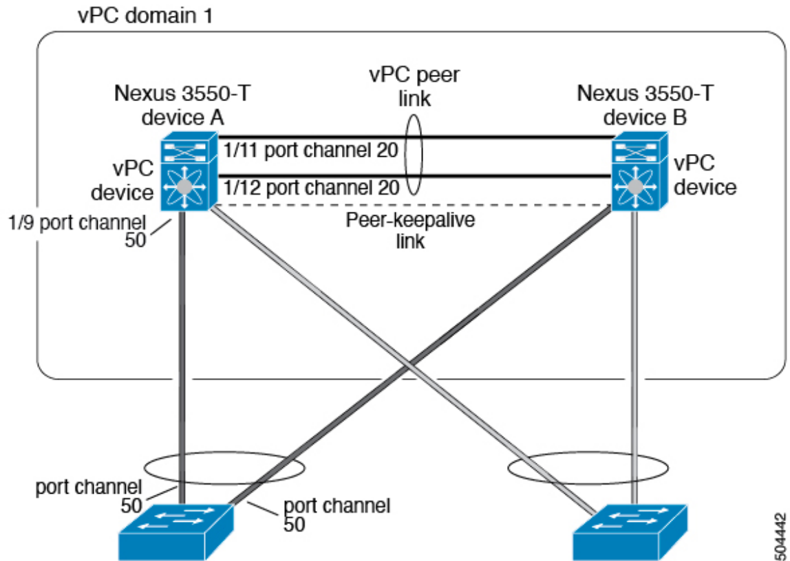
Figure 16: vPC Configuration Example
