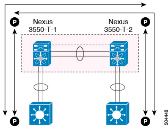
Figure 17: Peering Over a PC Interconnection and Dedicated Interswitch Link Using non-vPC VLAN
