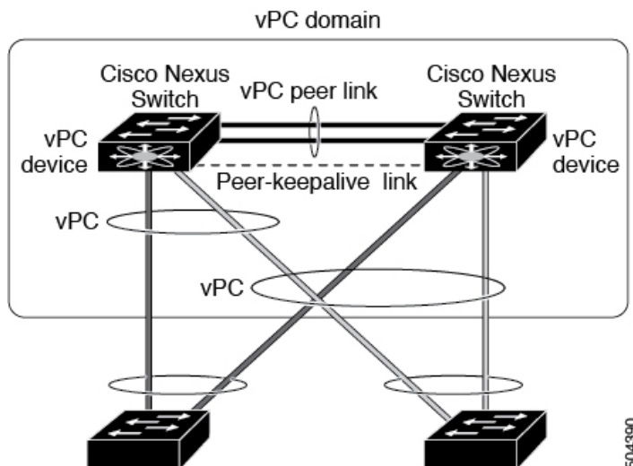
Figure 5: vPC Architecture
