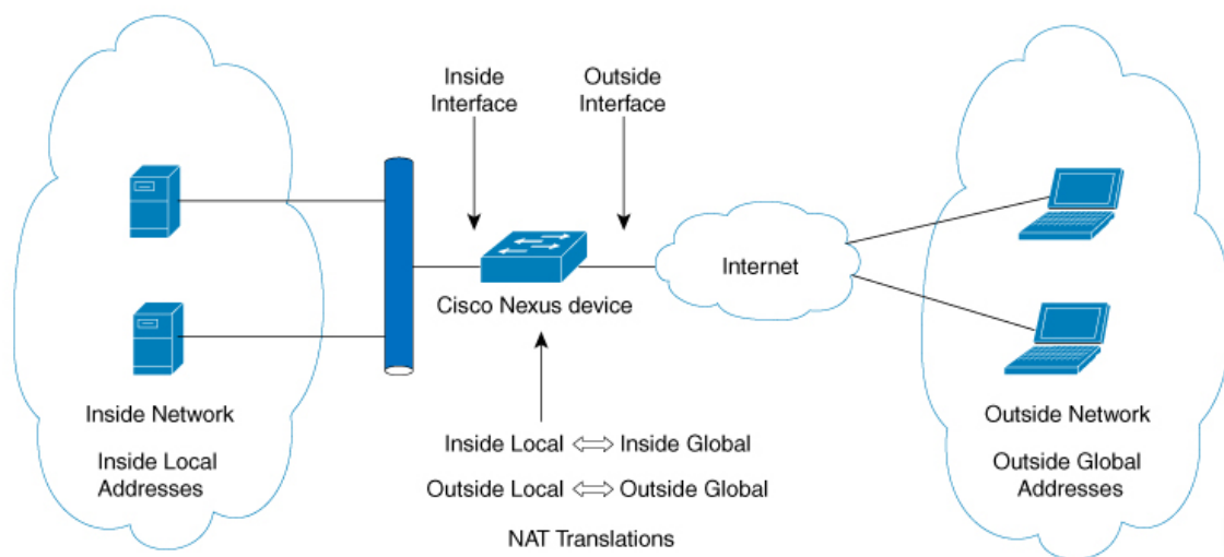
Figure 1: Static NAT
