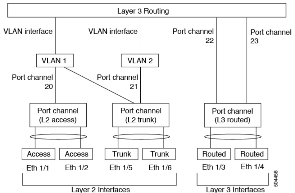
Figure 4: Port-Channel Interfaces
