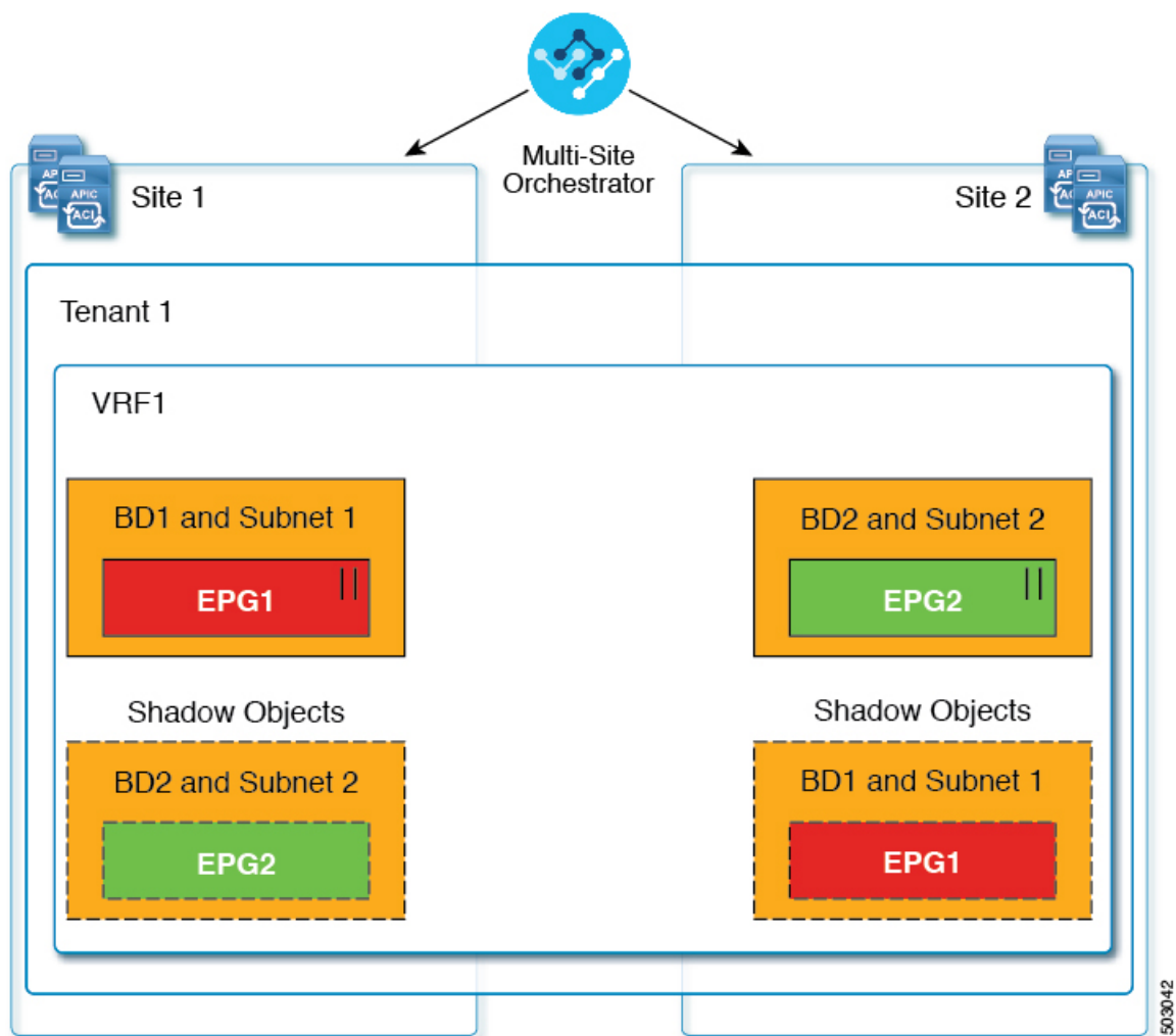
Figure 2: Preferred Group
