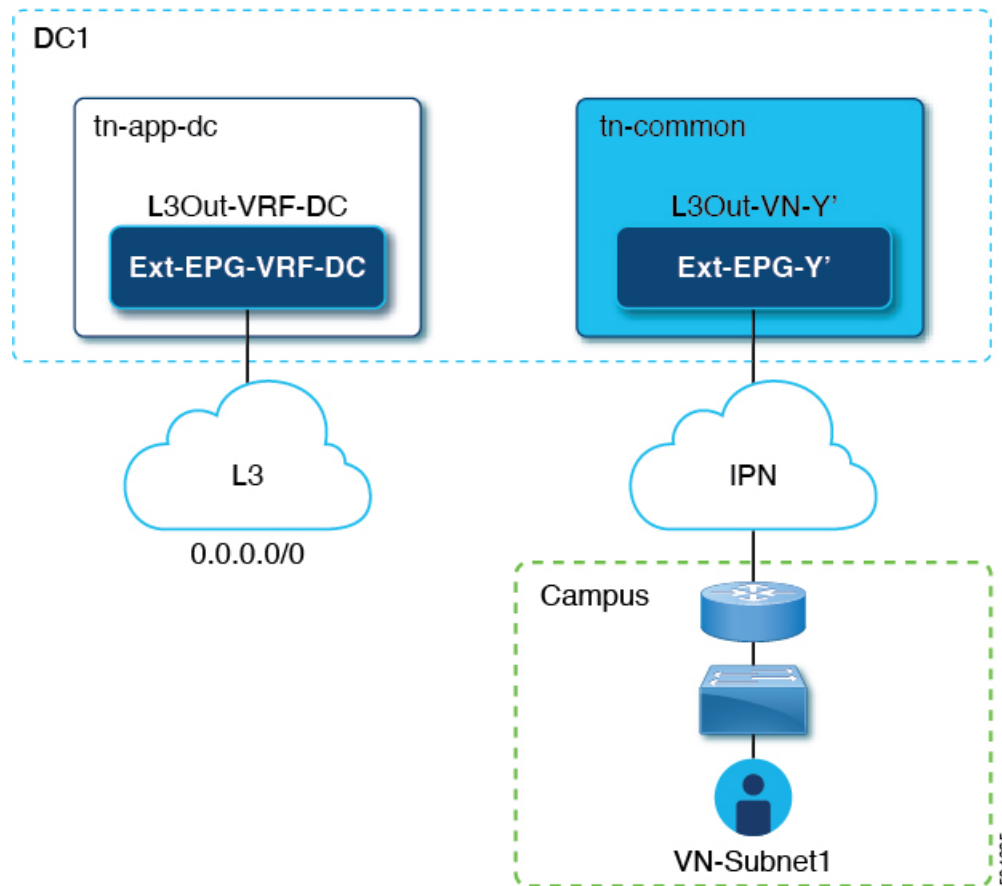
Figure 28: L3Out connection
