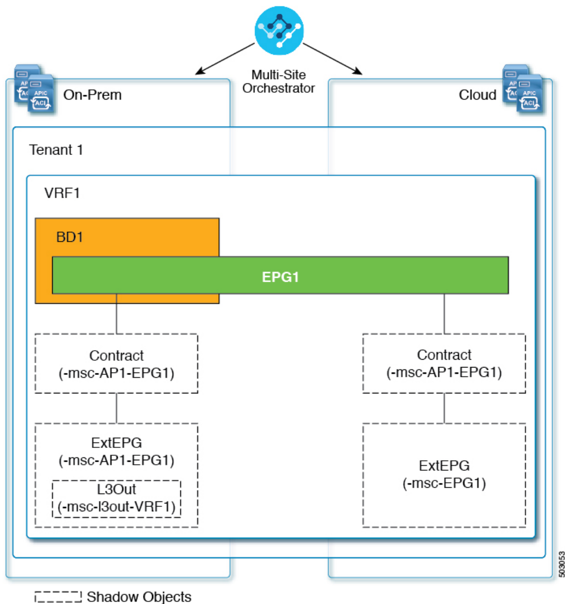
Figure 4: Hybrid Cloud
