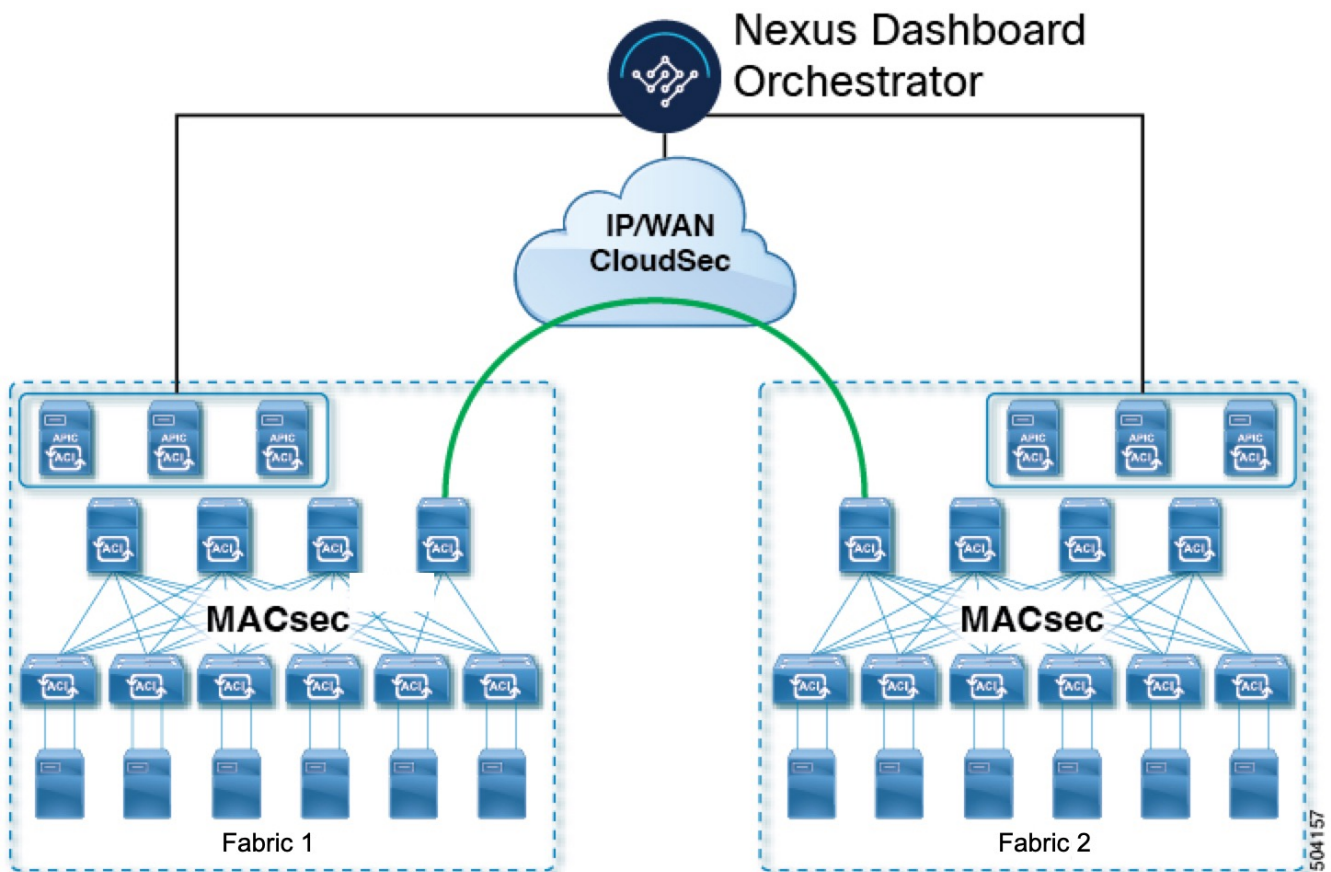
Figure 1. CloudSec Encryption
