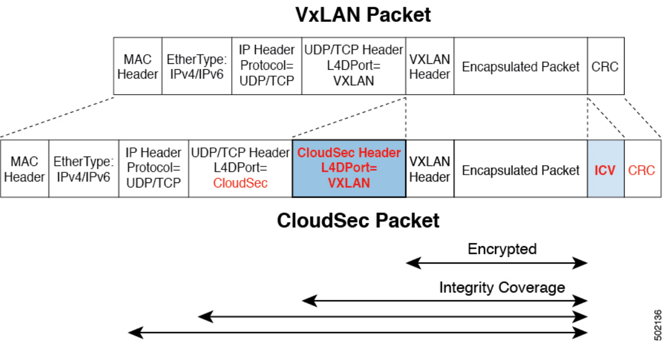
Figure 2. CloudSec Packet
