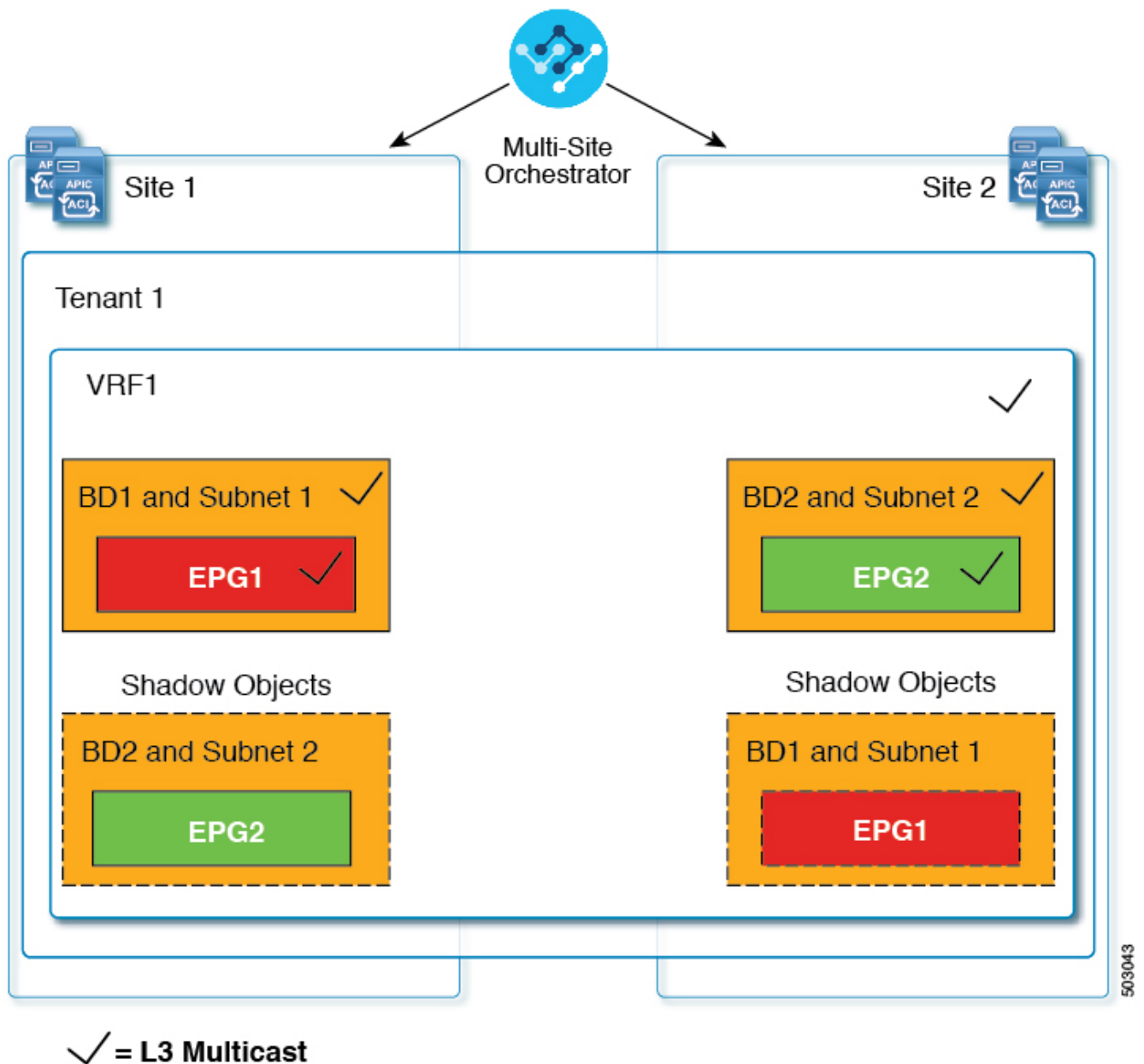
Figure 3. L3 Multicast
