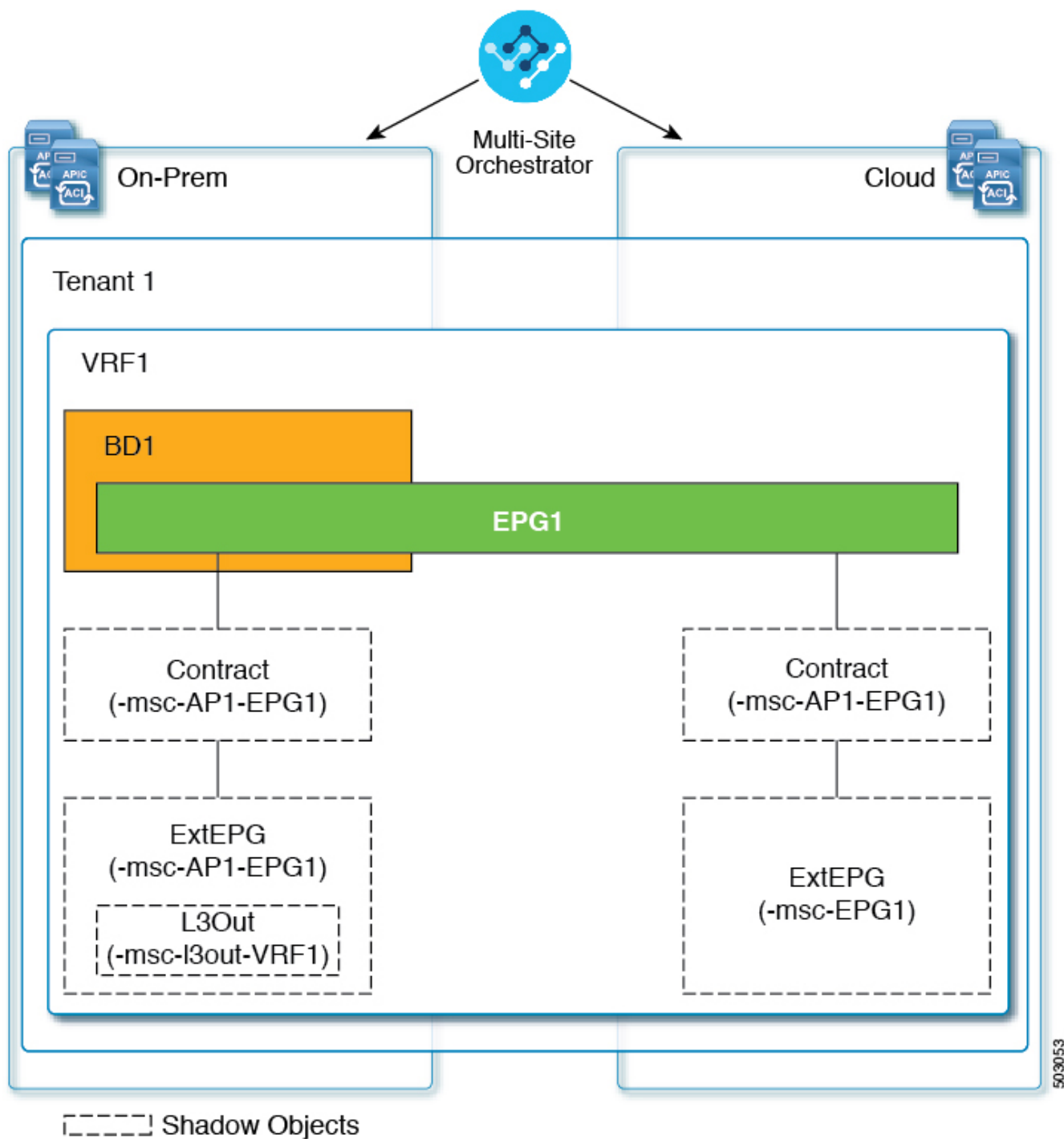
Figure 4. Hybrid Cloud
