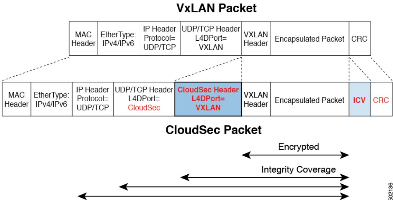
Figure 2. CloudSec Packet
