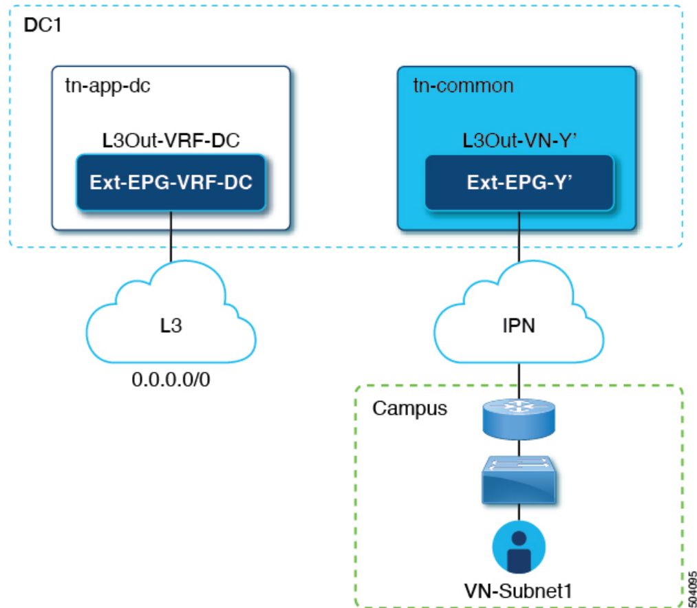
Figure 5: L3Out connection
