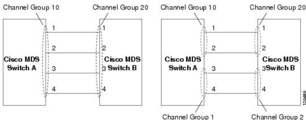
Figure 6: Valid Port Channel Configurations
