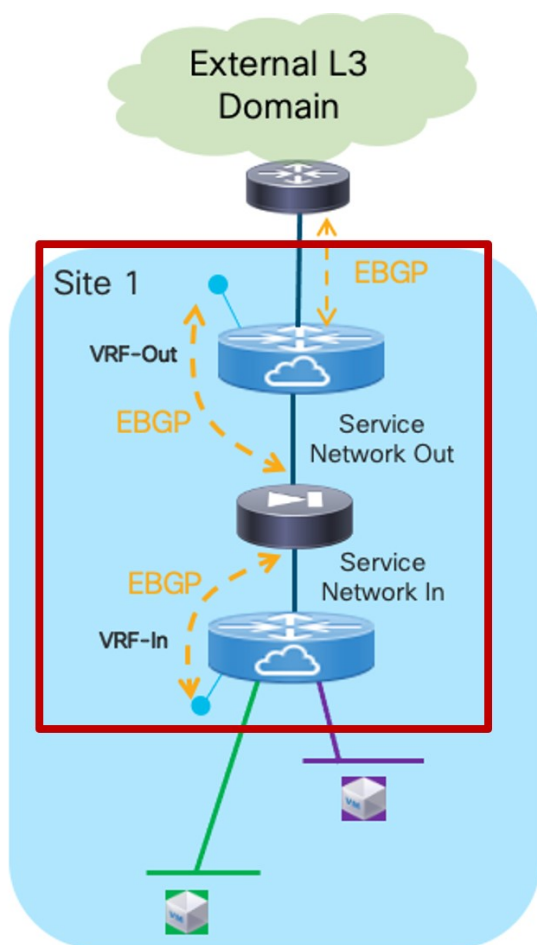
Service Function as Perimeter Device: Outside and Inside VRFs
