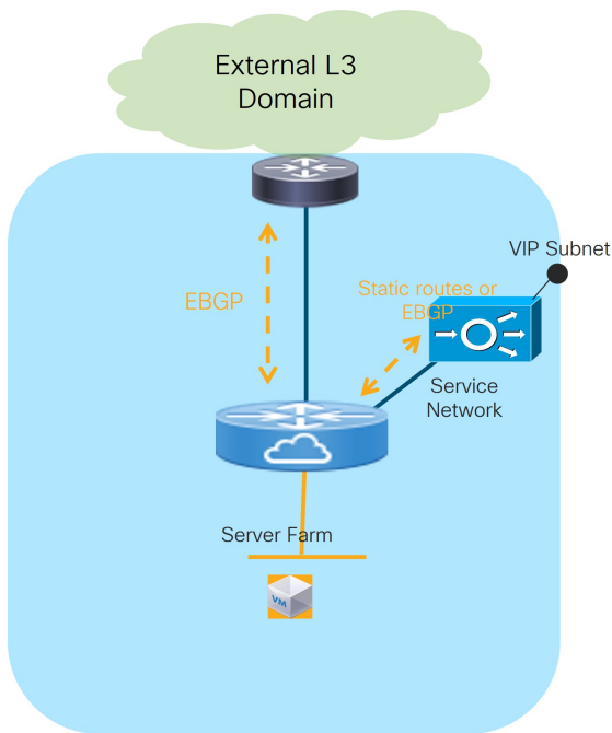
Load Balancer with Source NAT
