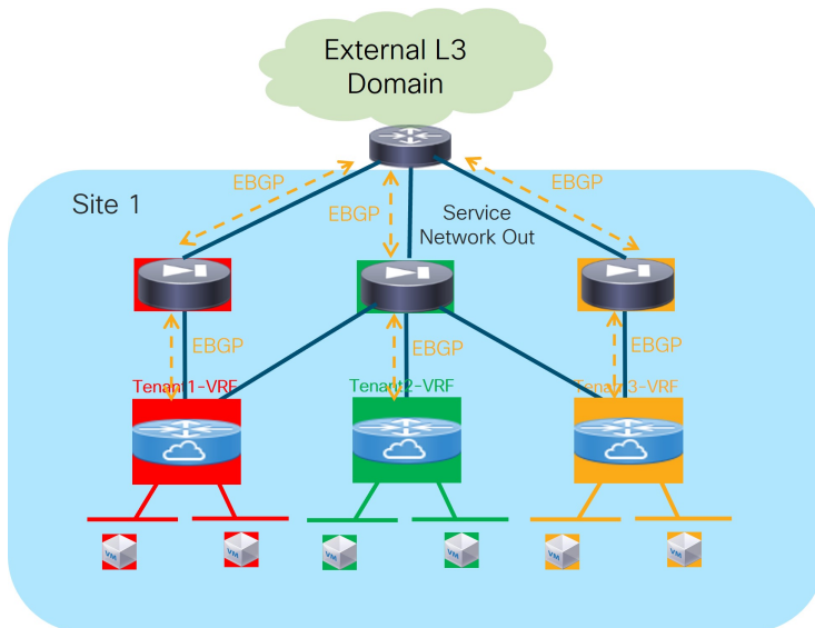
One Arm Perimeter Firewall
