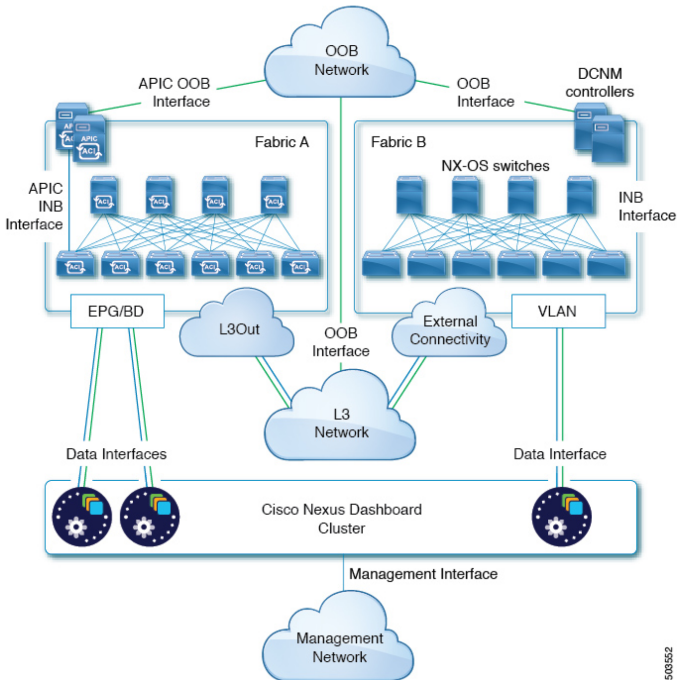
Connecting via an EPG/BD, Nexus Dashboard Orchestrator
