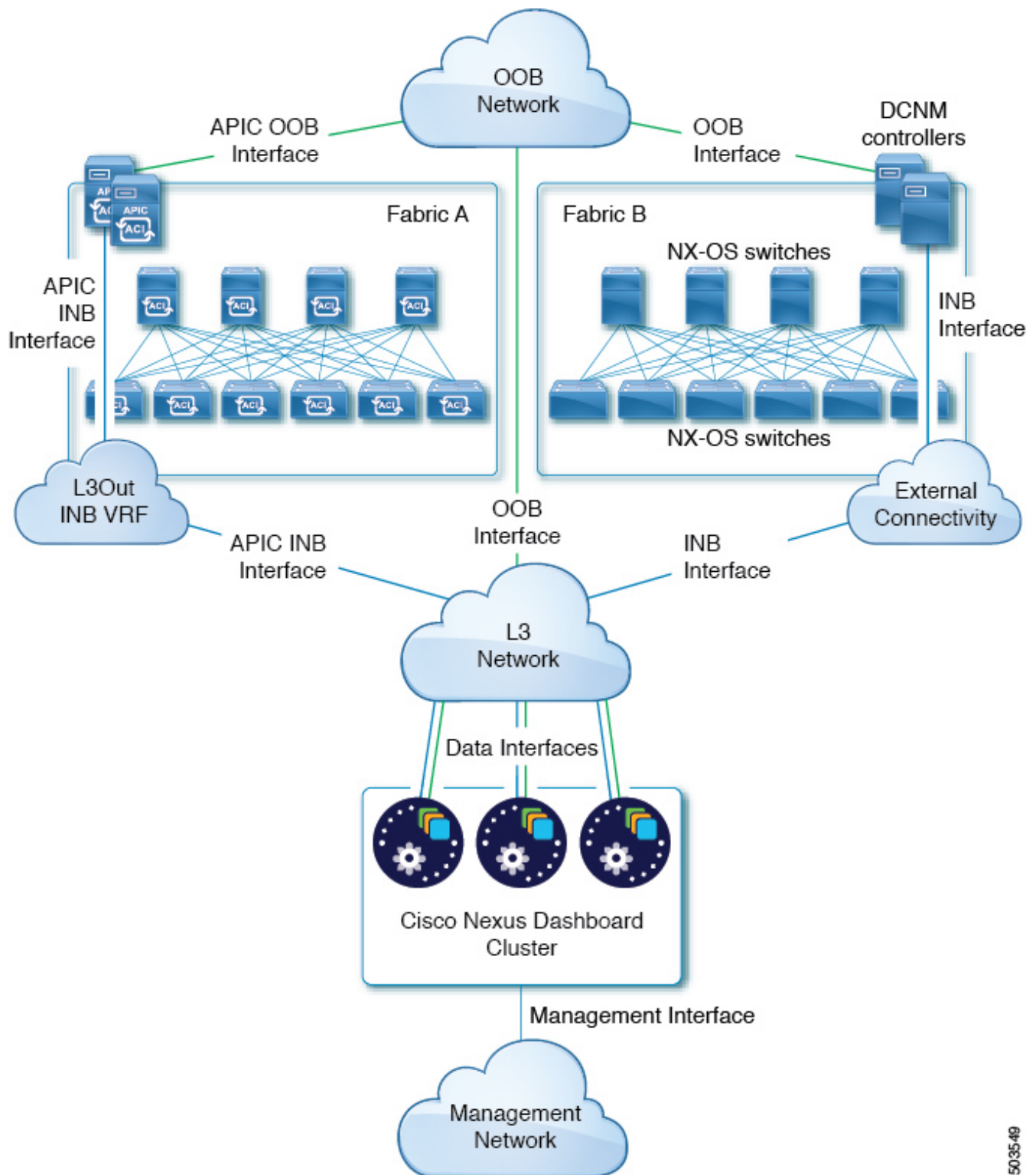
Connecting via External Layer 3 Network, Nexus Dashboard Orchestrator
