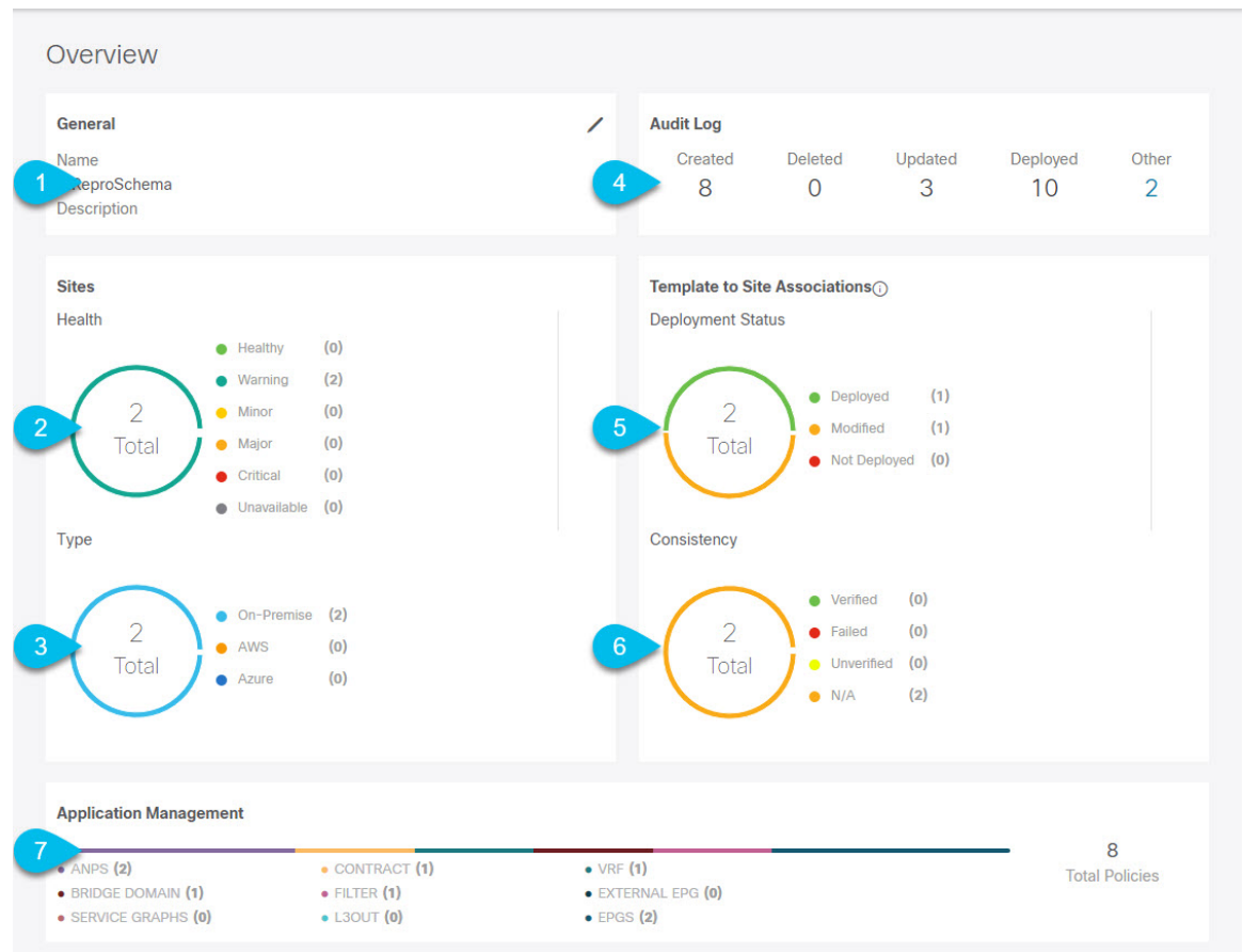
Figure 4: Schema Overview
