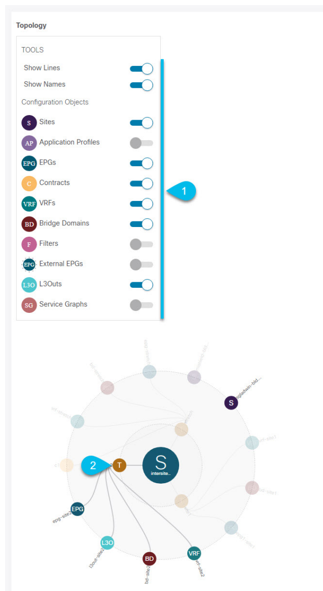
Figure 5: Deployment Visualizer
