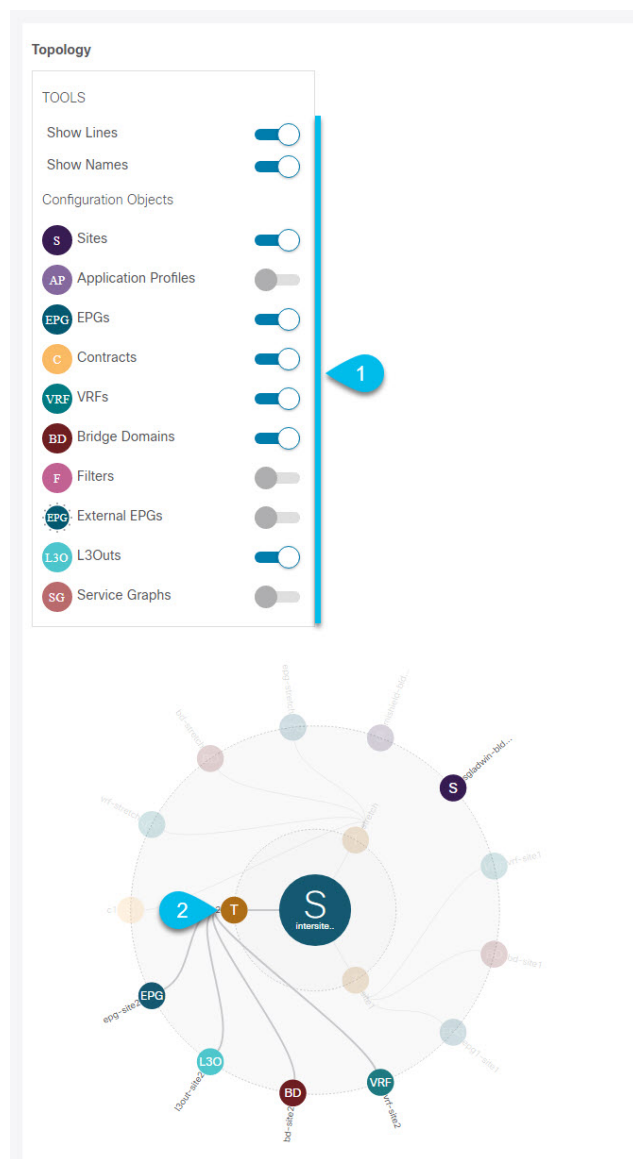
Figure 5: Deployment Visualizer
