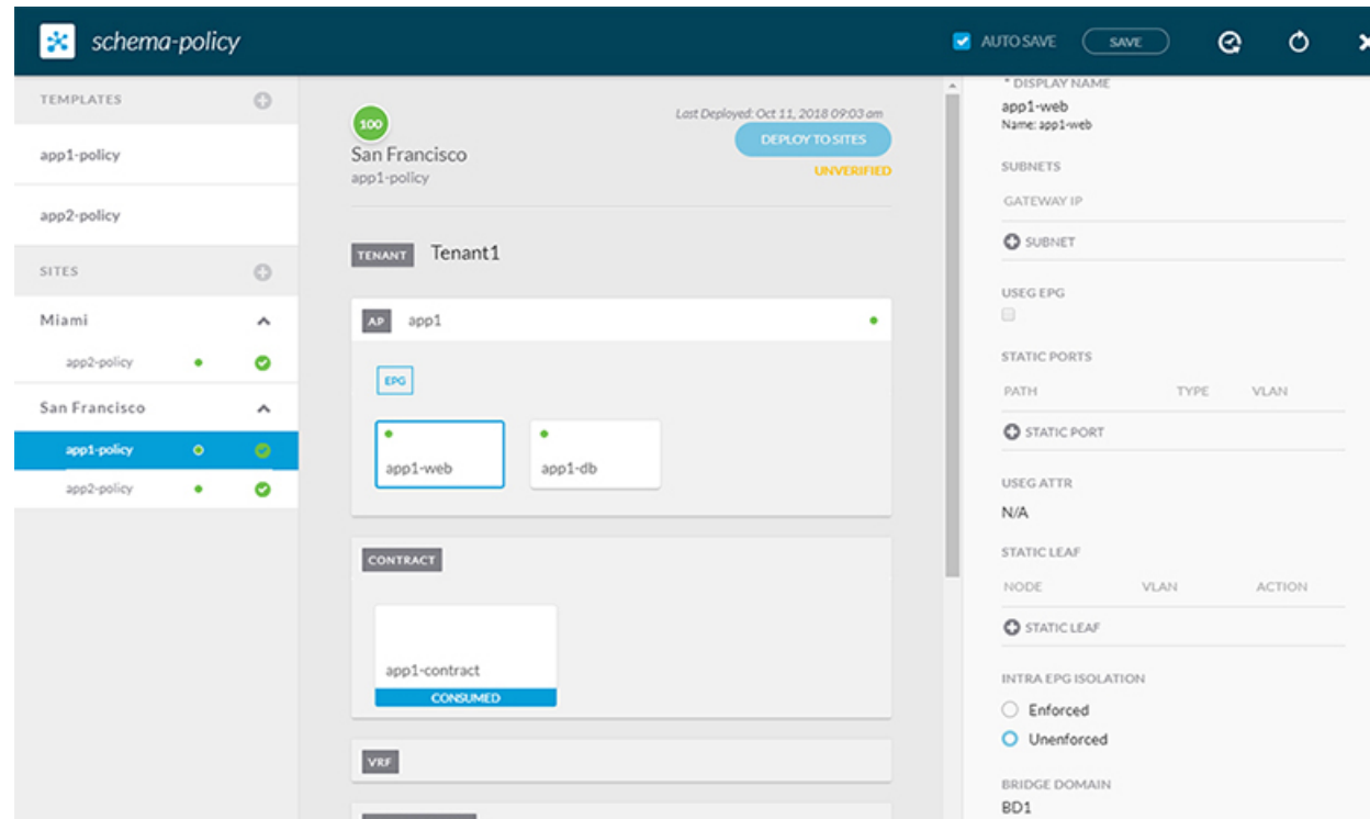
Figure 2: Policy Schema
