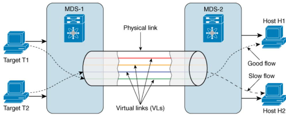
Figure 1: Traffic Flow Using Virtual Links
