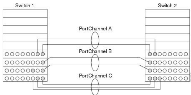
Figure 15: Port Channel Flexibility
