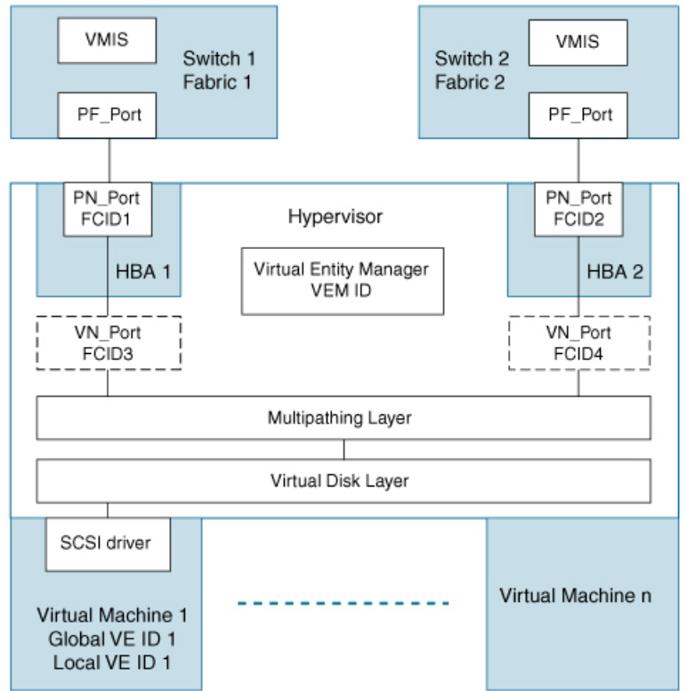
Figure 54: VE ID Life Cycle, on page 223 shows how VE ID changes during a VM life cycle:
