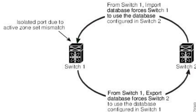
Figure 29: Importing and Exporting the Database
