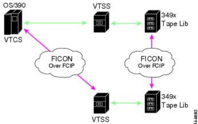
Figure 62: Host Accessing Peer-to-Peer VTS (Virtual Tape Server)
