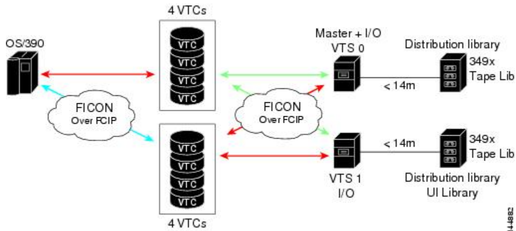
Figure 61: Host Accessing Peer-to-Peer VTS (Virtual Tape Server)
