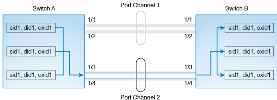
Figure 49: ECMP Hashing Method
