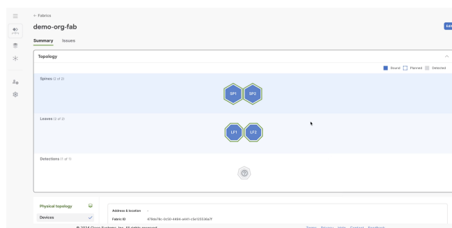
Figure 6: Bound switches
