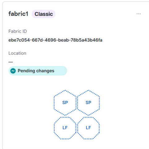
Figure 3: Pending changes
