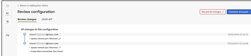
Figure 4: Review configuration
