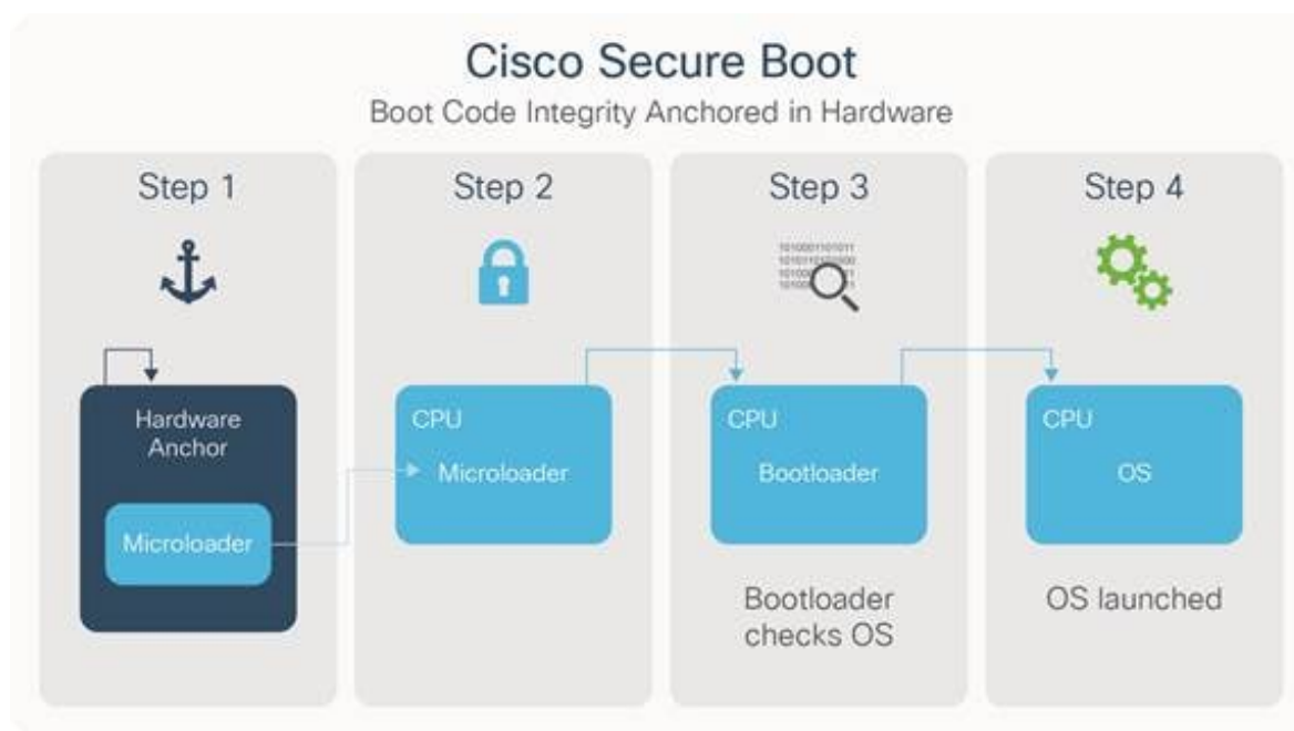
Figure 1: Workflow for boot code integrity and security in Cisco 6000 Series switches
