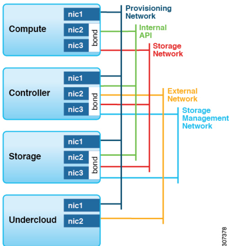
Figure 2: Typical topology for installation of Red Hat OpenStack Platform 16.2 with the Cisco ACI plug-in
