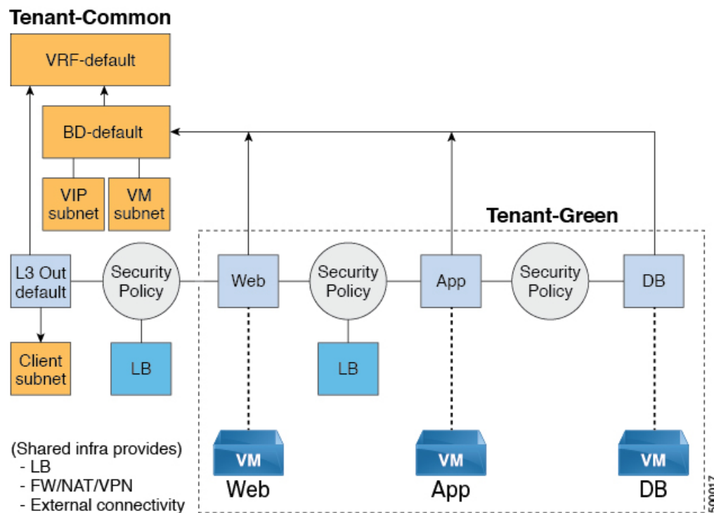
Figure 4: Shared Plan - Load Balancer Overview
